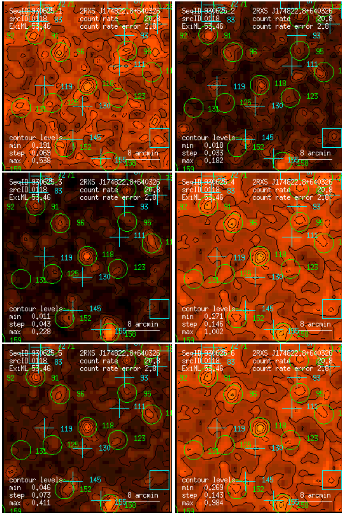
Figure 118: RASS 930625: detection 0118: band rate images, Gaussian filter: (1) PSPC channels 11 – 41, (2) 52 – 90, (3) 91 – 201, (4) 11 – 235, (5) 52 – 201, (6) 11 – 201. Broad band rates in counts/ks. Band rate contour levels in counts/ks/arcmin 2 .
