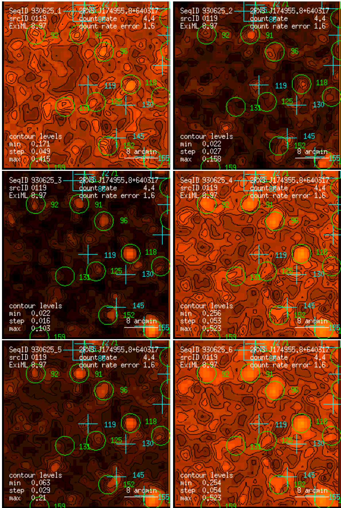
Figure 119: RASS 930625: detection 0119: band rate images, Gaussian filter: (1) PSPC channels 11 – 41, (2) 52 – 90, (3) 91 – 201, (4) 11 – 235, (5) 52 – 201, (6) 11 – 201. Broad band rates in counts/ks. Band rate contour levels in counts/ks/arcmin 2 .
