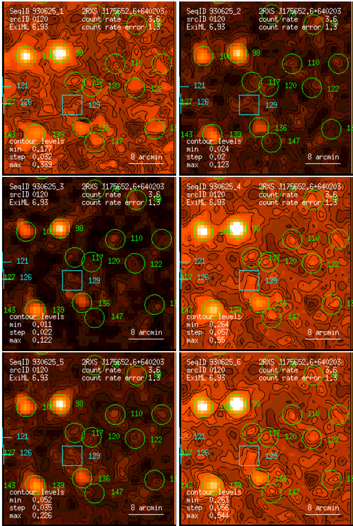
Figure 120: RASS 930625: detection 0120: band rate images, Gaussian filter: (1) PSPC channels 11 – 41, (2) 52 – 90, (3) 91 – 201, (4) 11 – 235, (5) 52 – 201, (6) 11 – 201. Broad band rates in counts/ks. Band rate contour levels in counts/ks/arcmin 2 .
