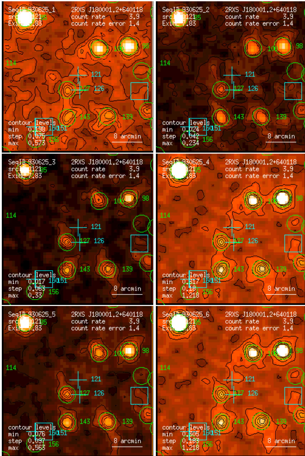
Figure 121: RASS 930625: detection 0121: band rate images, Gaussian filter: (1) PSPC channels 11 – 41, (2) 52 – 90, (3) 91 – 201, (4) 11 – 235, (5) 52 – 201, (6) 11 – 201. Broad band rates in counts/ks. Band rate contour levels in counts/ks/arcmin 2 .
