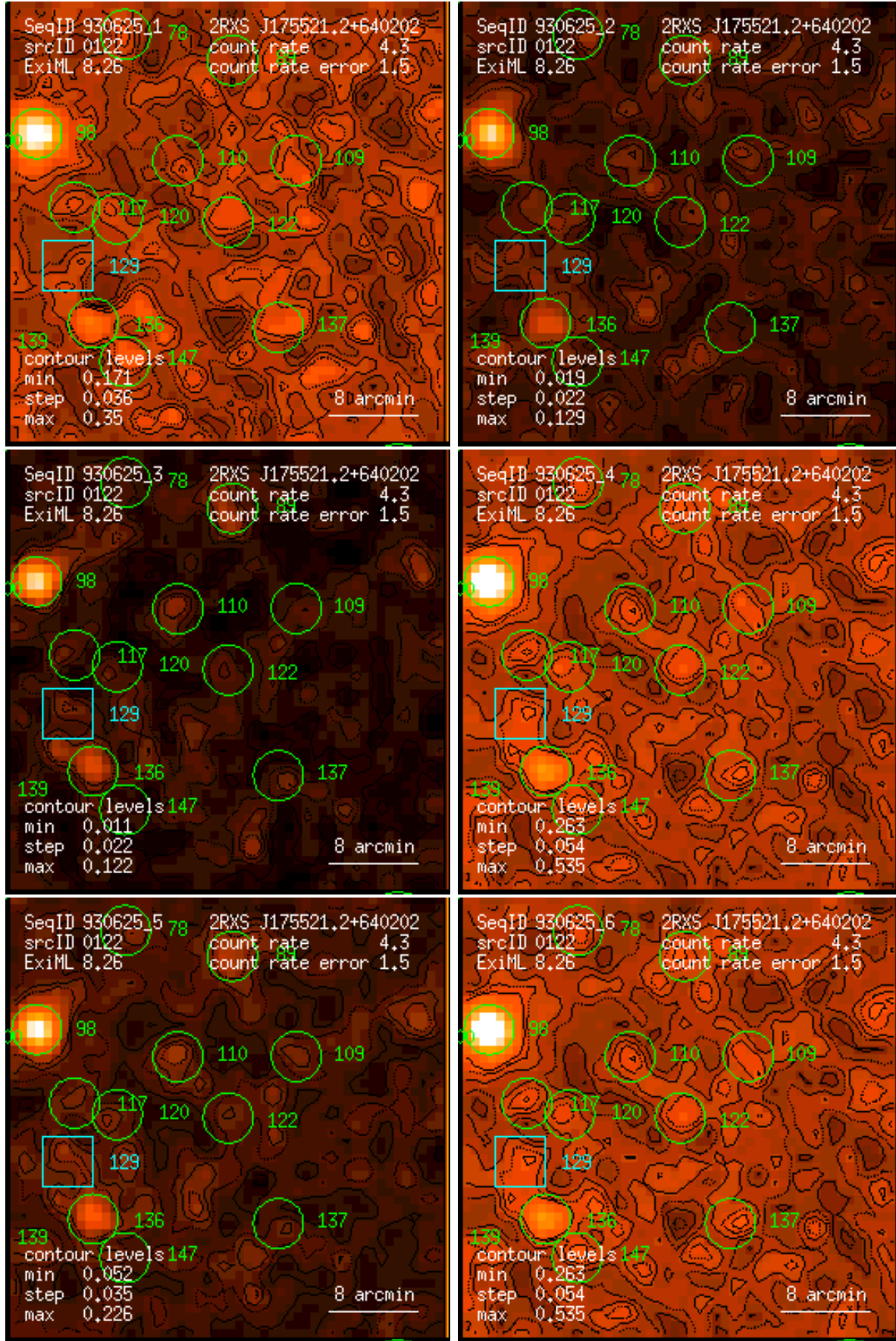
Figure 122: RASS 930625: detection 0122: band rate images, Gaussian filter: (1) PSPC channels 11 – 41, (2) 52 – 90, (3) 91 – 201, (4) 11 – 235, (5) 52 – 201, (6) 11 – 201. Broad band rates in counts/ks. Band rate contour levels in counts/ks/arcmin 2 .
