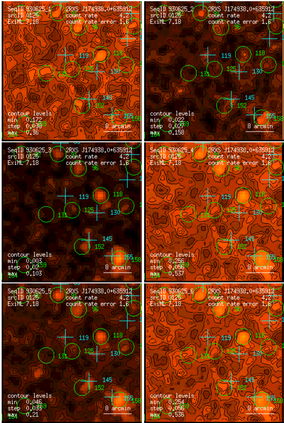
Figure 125: RASS 930625: detection 0125: band rate images, Gaussian filter: (1) PSPC channels 11 – 41, (2) 52 – 90, (3) 91 – 201, (4) 11 – 235, (5) 52 – 201, (6) 11 – 201. Broad band rates in counts/ks. Band rate contour levels in counts/ks/arcmin 2 .
