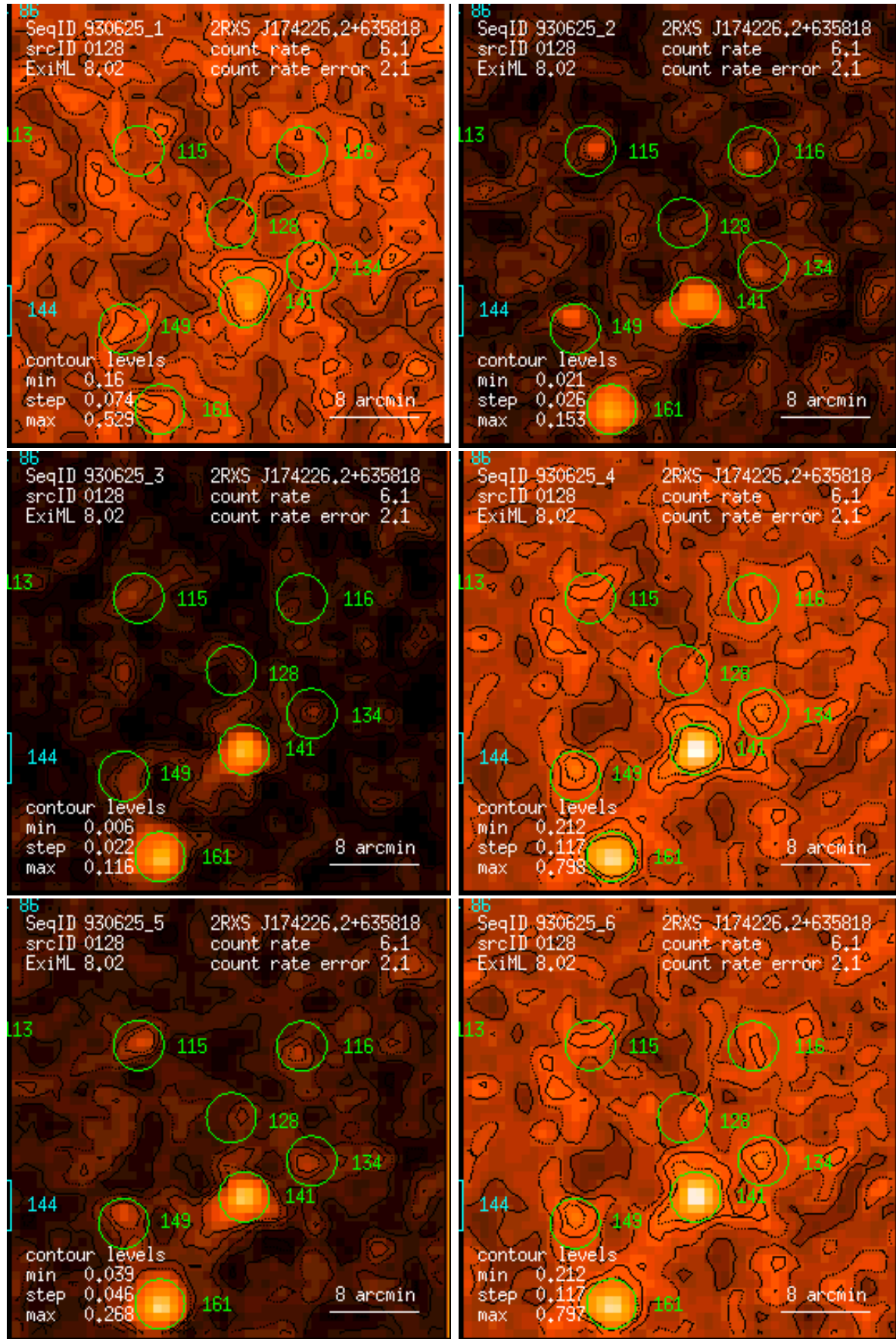
Figure 128: RASS 930625: detection 0128: band rate images, Gaussian filter: (1) PSPC channels 11 – 41, (2) 52 – 90, (3) 91 – 201, (4) 11 – 235, (5) 52 – 201, (6) 11 – 201. Broad band rates in counts/ks. Band rate contour levels in counts/ks/arcmin 2 .
