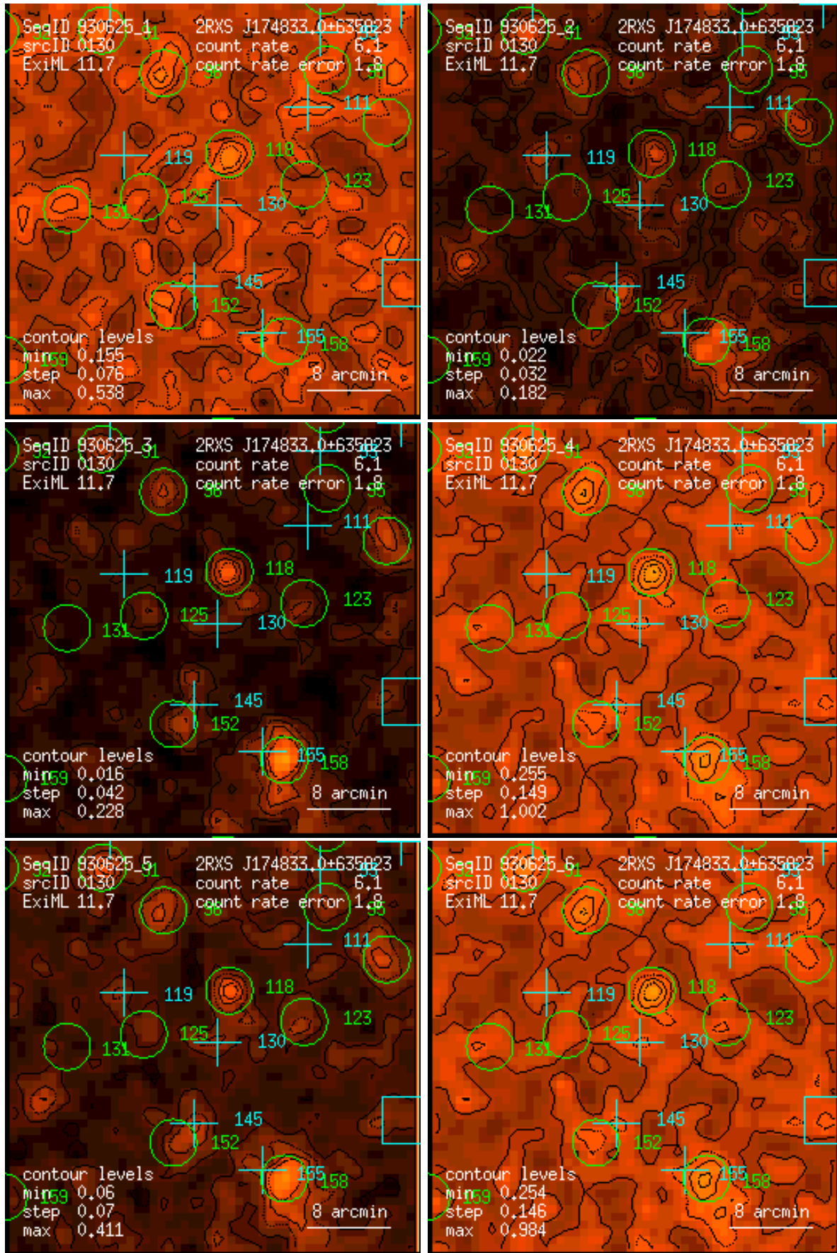
Figure 130: RASS 930625: detection 0130: band rate images, Gaussian filter: (1) PSPC channels 11 – 41, (2) 52 – 90, (3) 91 – 201, (4) 11 – 235, (5) 52 – 201, (6) 11 – 201. Broad band rates in counts/ks. Band rate contour levels in counts/ks/arcmin 2 .
