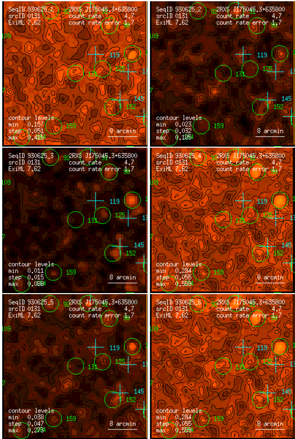
Figure 131: RASS 930625: detection 0131: band rate images, Gaussian filter: (1) PSPC channels 11 – 41, (2) 52 – 90, (3) 91 – 201, (4) 11 – 235, (5) 52 – 201, (6) 11 – 201. Broad band rates in counts/ks. Band rate contour levels in counts/ks/arcmin 2 .
