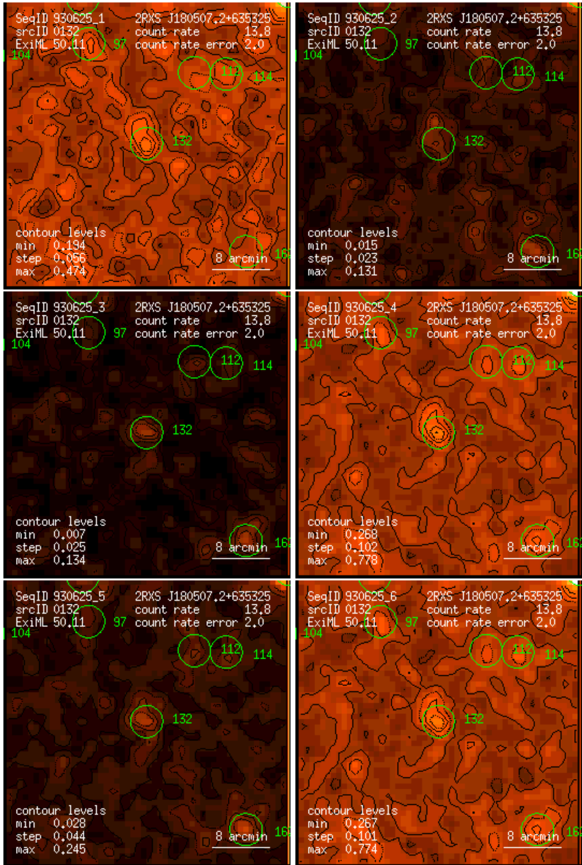
Figure 132: RASS 930625: detection 0132: band rate images, Gaussian filter: (1) PSPC channels 11 – 41, (2) 52 – 90, (3) 91 – 201, (4) 11 – 235, (5) 52 – 201, (6) 11 – 201. Broad band rates in counts/ks. Band rate contour levels in counts/ks/arcmin 2 .
