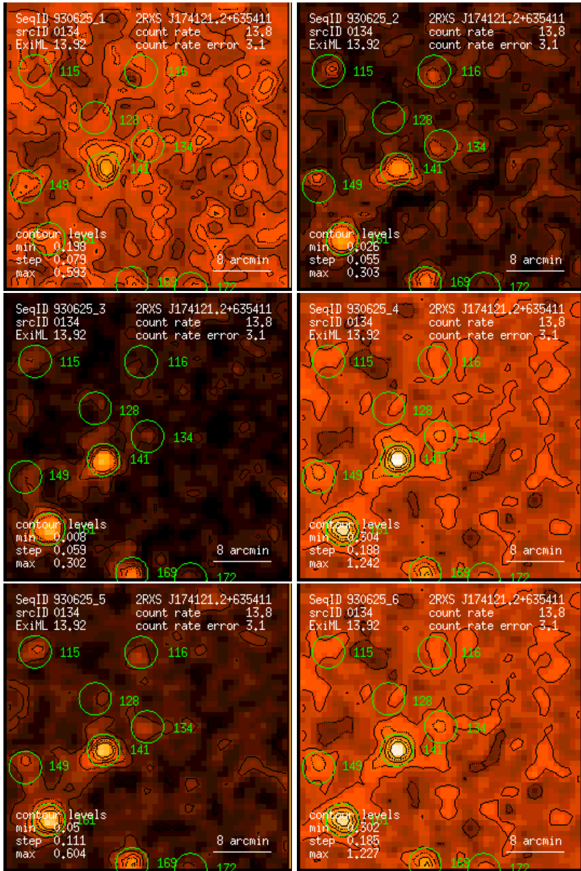
Figure 134: RASS 930625: detection 0134: band rate images, Gaussian filter: (1) PSPC channels 11 – 41, (2) 52 – 90, (3) 91 – 201, (4) 11 – 235, (5) 52 – 201, (6) 11 – 201. Broad band rates in counts/ks. Band rate contour levels in counts/ks/arcmin 2 .
