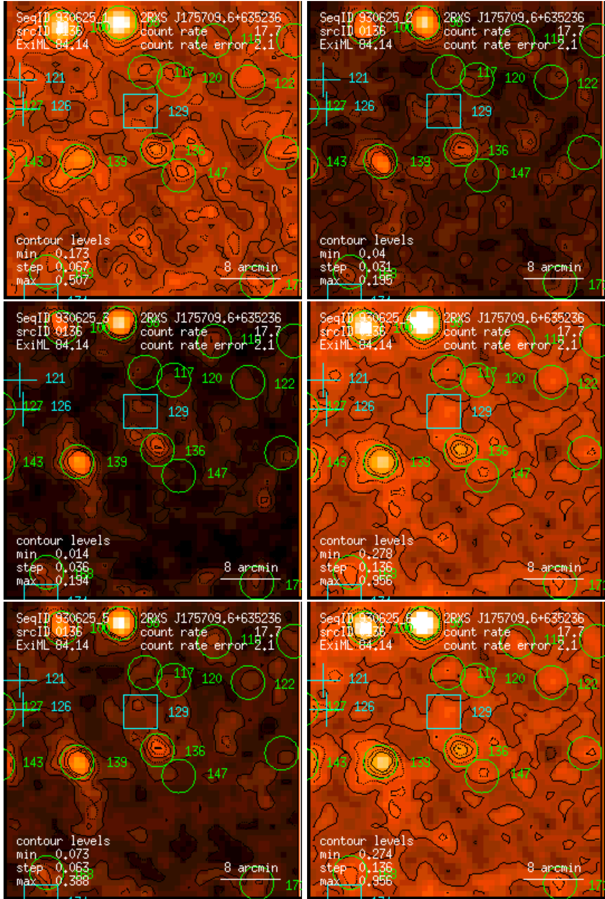
Figure 136: RASS 930625: detection 0136: band rate images, Gaussian filter: (1) PSPC channels 11 – 41, (2) 52 – 90, (3) 91 – 201, (4) 11 – 235, (5) 52 – 201, (6) 11 – 201. Broad band rates in counts/ks. Band rate contour levels in counts/ks/arcmin 2 .
