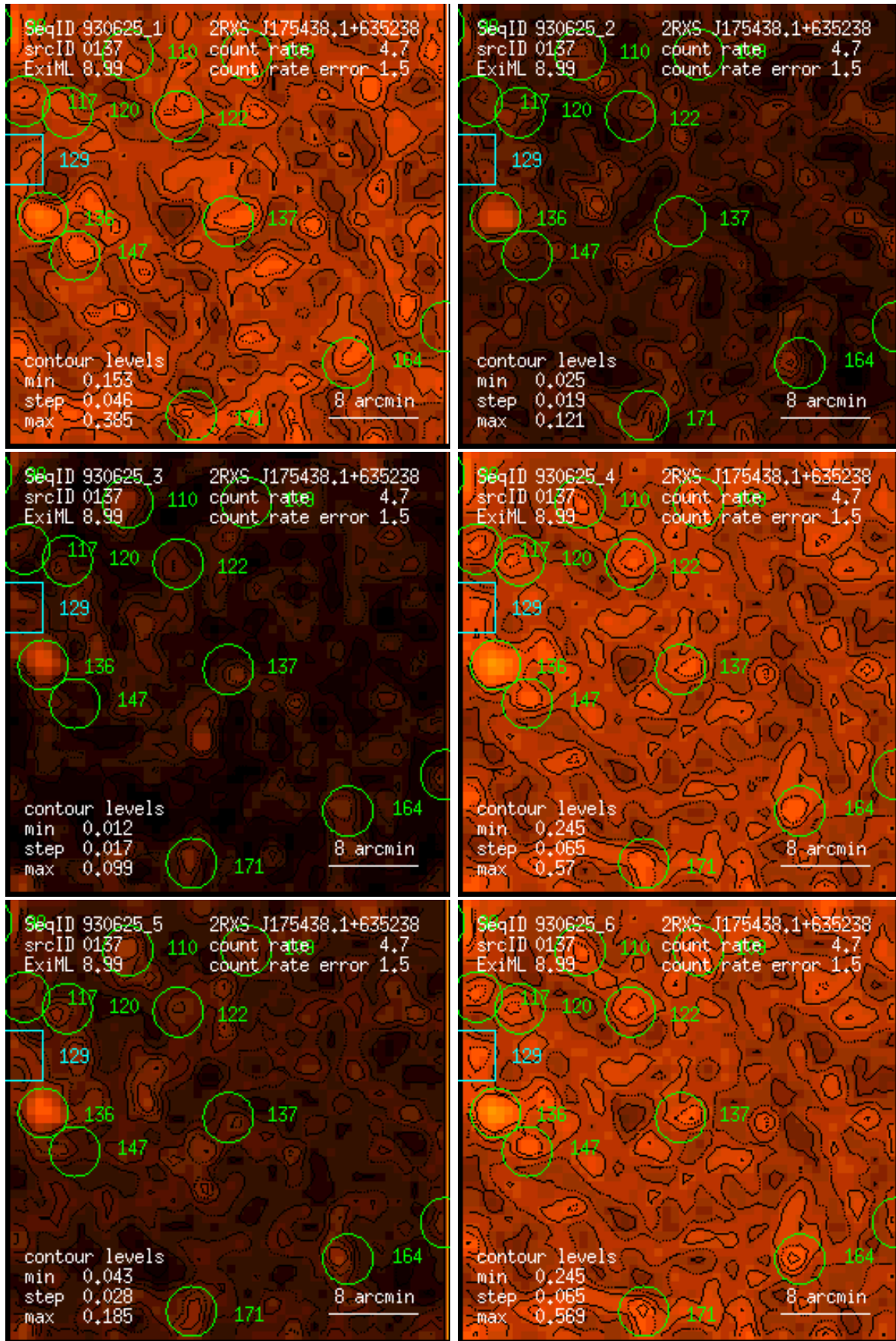
Figure 137: RASS 930625: detection 0137: band rate images, Gaussian filter: (1) PSPC channels 11 – 41, (2) 52 – 90, (3) 91 – 201, (4) 11 – 235, (5) 52 – 201, (6) 11 – 201. Broad band rates in counts/ks. Band rate contour levels in counts/ks/arcmin 2 .
