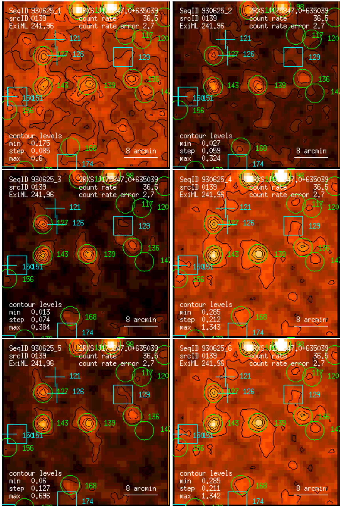
Figure 139: RASS 930625: detection 0139: band rate images, Gaussian filter: (1) PSPC channels 11 – 41, (2) 52 – 90, (3) 91 – 201, (4) 11 – 235, (5) 52 – 201, (6) 11 – 201. Broad band rates in counts/ks. Band rate contour levels in counts/ks/arcmin 2 .
