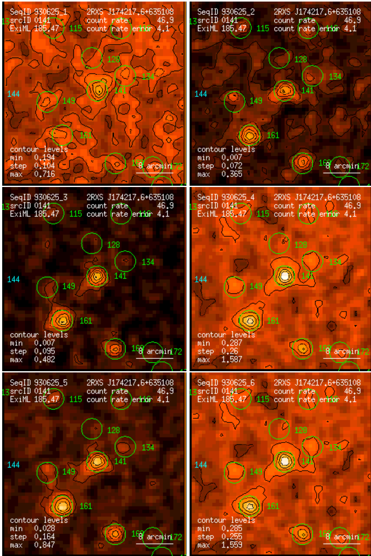
Figure 141: RASS 930625: detection 0141: band rate images, Gaussian filter: (1) PSPC channels 11 – 41, (2) 52 – 90, (3) 91 – 201, (4) 11 – 235, (5) 52 – 201, (6) 11 – 201. Broad band rates in counts/ks. Band rate contour levels in counts/ks/arcmin 2 .
