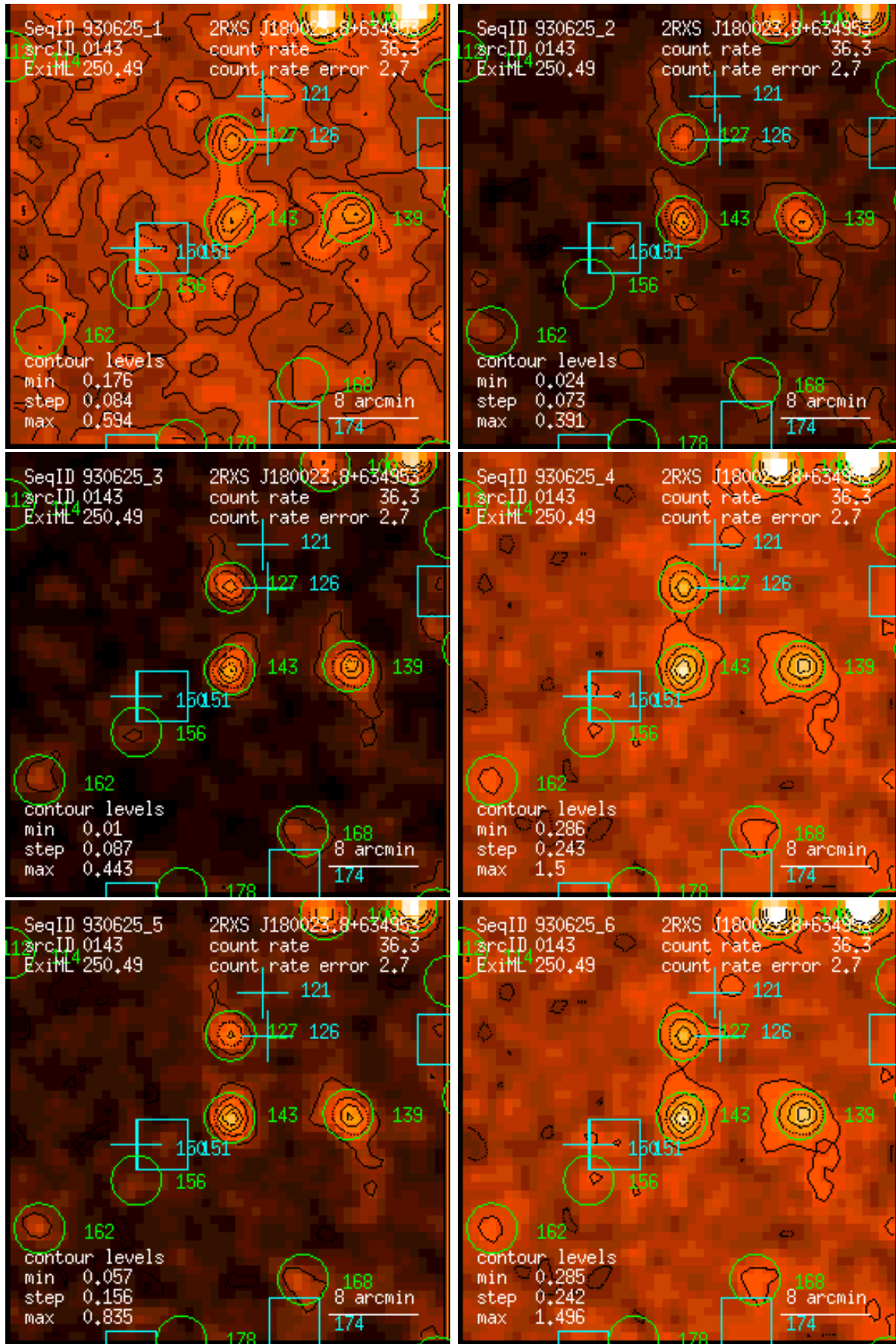
Figure 143: RASS 930625: detection 0143: band rate images, Gaussian filter: (1) PSPC channels 11 – 41, (2) 52 – 90, (3) 91 – 201, (4) 11 – 235, (5) 52 – 201, (6) 11 – 201. Broad band rates in counts/ks. Band rate contour levels in counts/ks/arcmin 2 .
