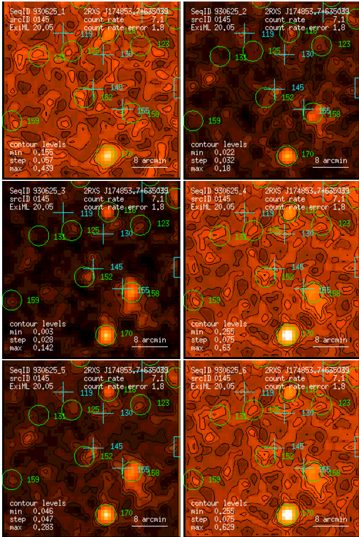
Figure 145: RASS 930625: detection 0145: band rate images, Gaussian filter: (1) PSPC channels 11 – 41, (2) 52 – 90, (3) 91 – 201, (4) 11 – 235, (5) 52 – 201, (6) 11 – 201. Broad band rates in counts/ks. Band rate contour levels in counts/ks/arcmin 2 .
