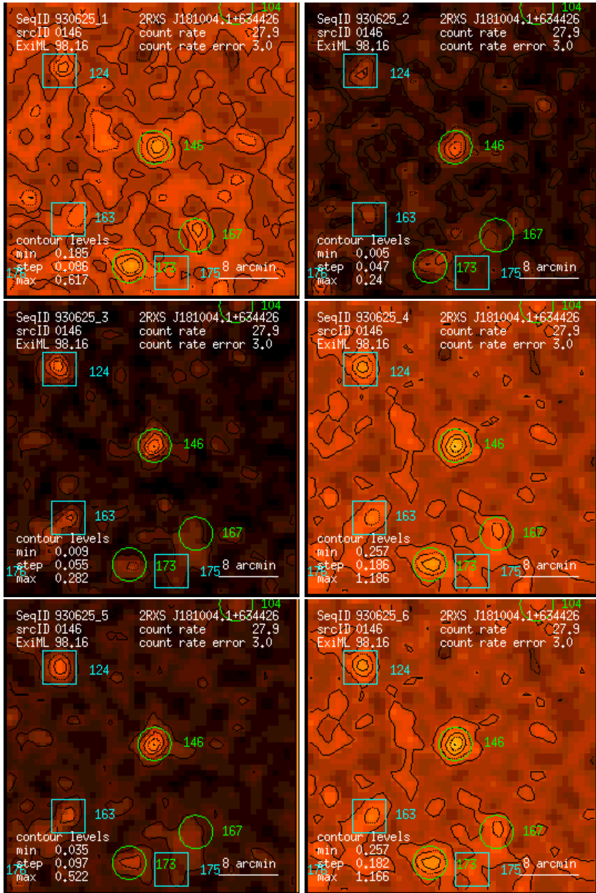
Figure 146: RASS 930625: detection 0146: band rate images, Gaussian filter: (1) PSPC channels 11 – 41, (2) 52 – 90, (3) 91 – 201, (4) 11 – 235, (5) 52 – 201, (6) 11 – 201. Broad band rates in counts/ks. Band rate contour levels in counts/ks/arcmin 2 .
