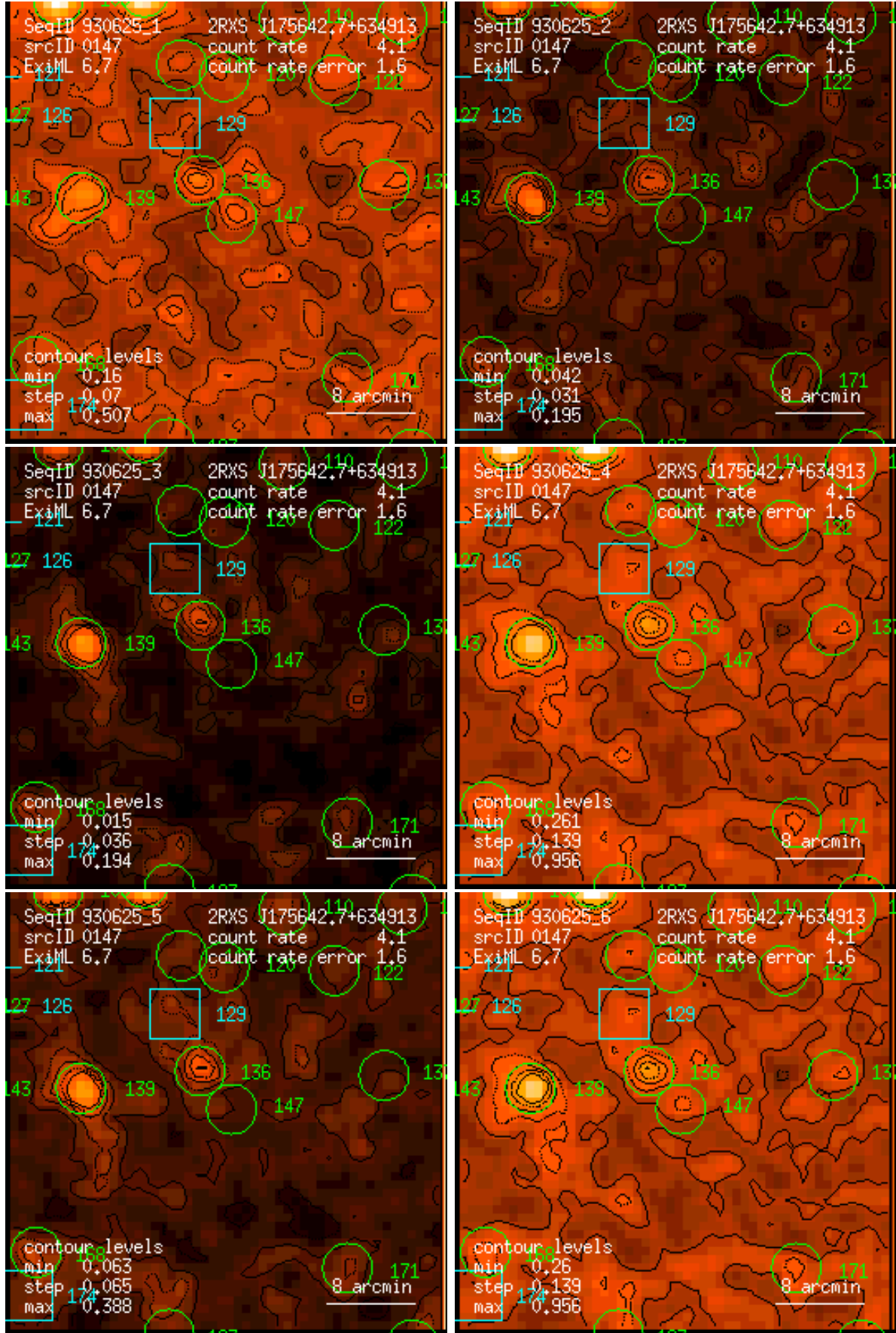
Figure 147: RASS 930625: detection 0147: band rate images, Gaussian filter: (1) PSPC channels 11 – 41, (2) 52 – 90, (3) 91 – 201, (4) 11 – 235, (5) 52 – 201, (6) 11 – 201. Broad band rates in counts/ks. Band rate contour levels in counts/ks/arcmin 2 .
