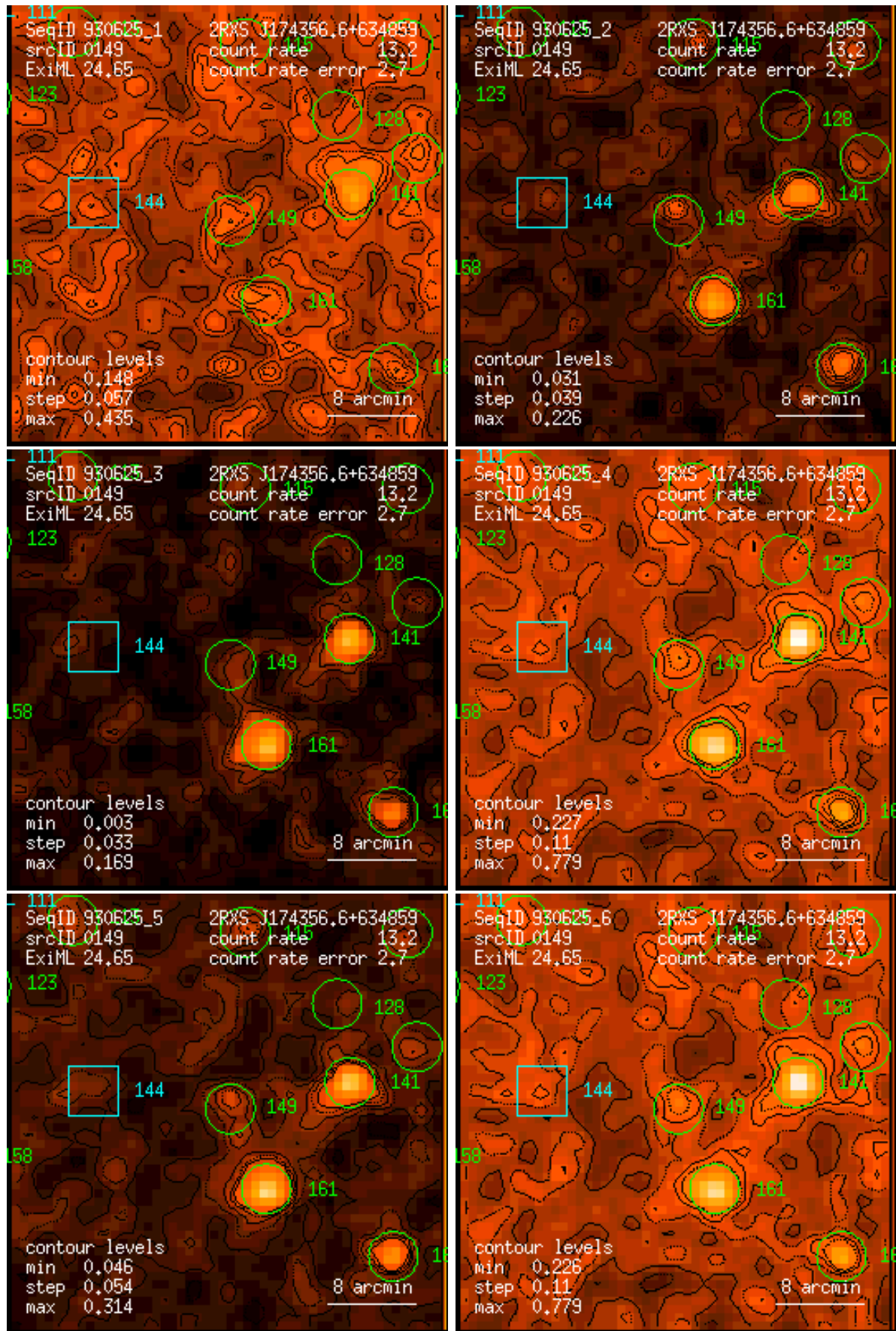
Figure 149: RASS 930625: detection 0149: band rate images, Gaussian filter: (1) PSPC channels 11 – 41, (2) 52 – 90, (3) 91 – 201, (4) 11 – 235, (5) 52 – 201, (6) 11 – 201. Broad band rates in counts/ks. Band rate contour levels in counts/ks/arcmin 2 .
