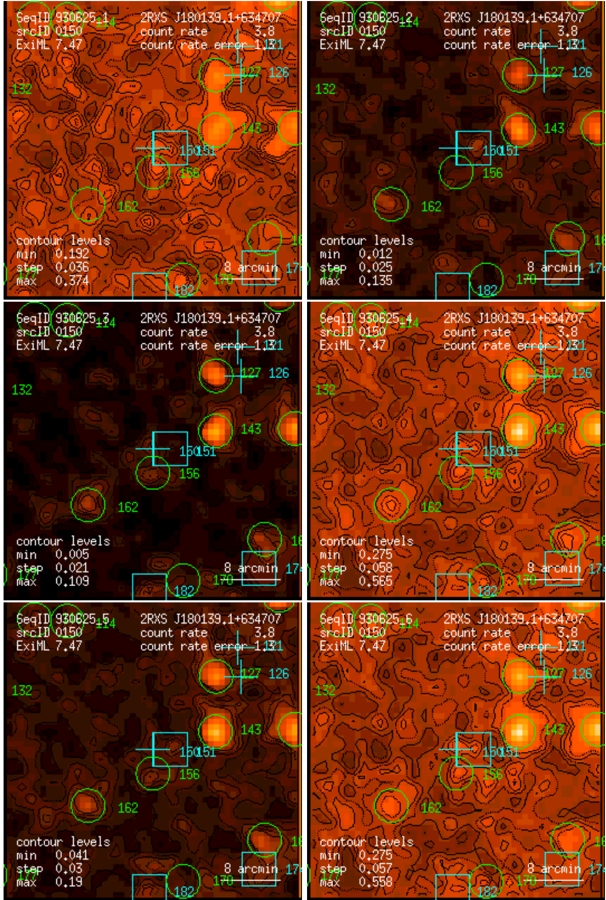
Figure 150: RASS 930625: detection 0150: band rate images, Gaussian filter: (1) PSPC channels 11 – 41, (2) 52 – 90, (3) 91 – 201, (4) 11 – 235, (5) 52 – 201, (6) 11 – 201. Broad band rates in counts/ks. Band rate contour levels in counts/ks/arcmin 2 .
