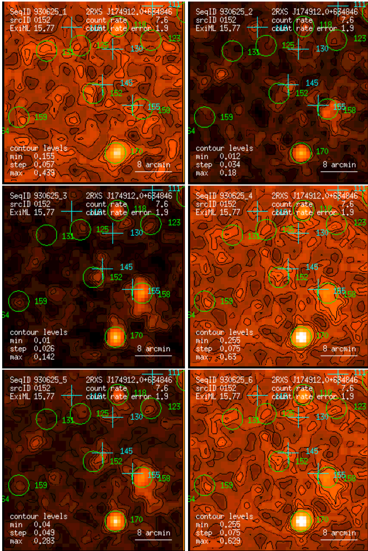
Figure 152: RASS 930625: detection 0152: band rate images, Gaussian filter: (1) PSPC channels 11 – 41, (2) 52 – 90, (3) 91 – 201, (4) 11 – 235, (5) 52 – 201, (6) 11 – 201. Broad band rates in counts/ks. Band rate contour levels in counts/ks/arcmin 2 .
