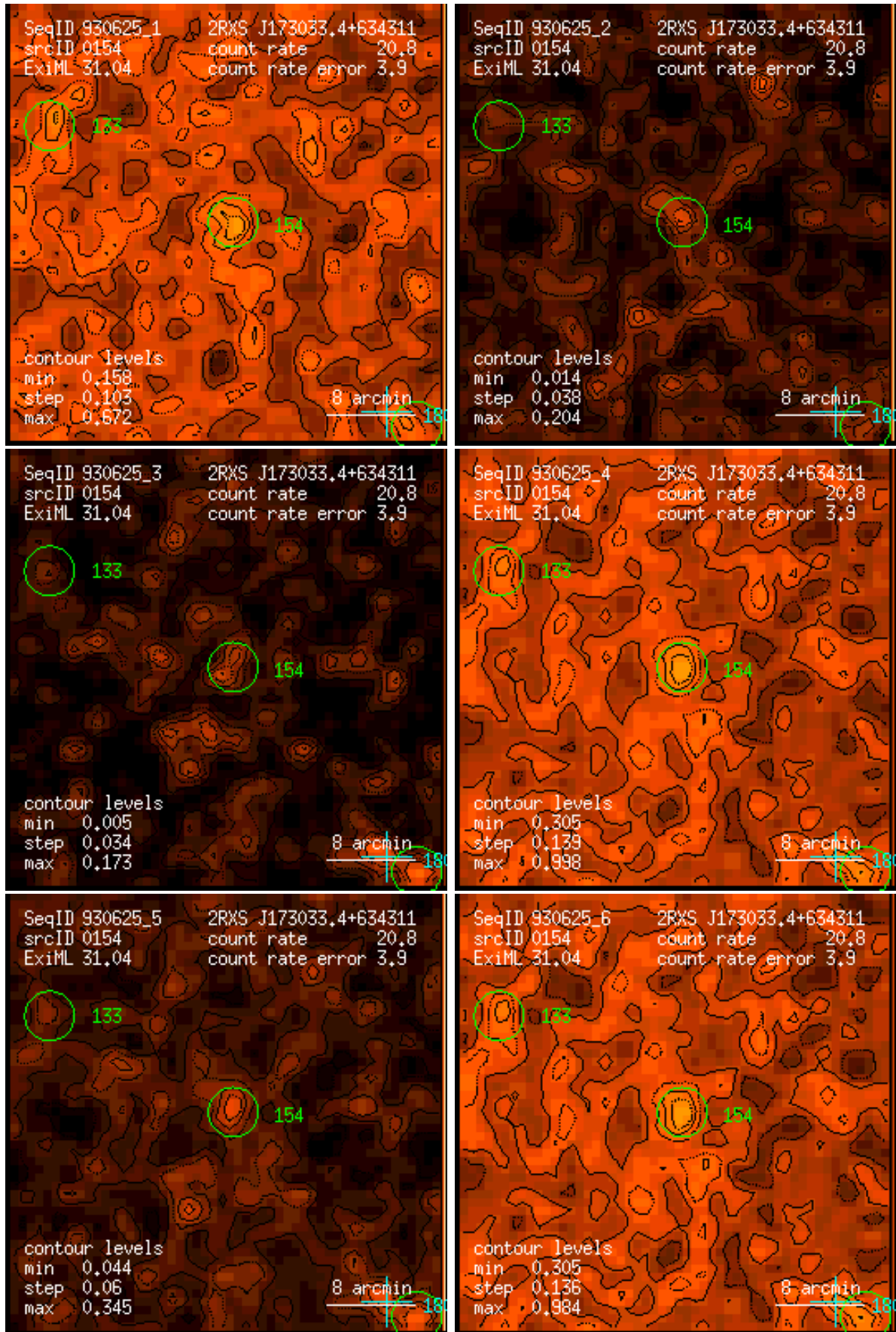
Figure 154: RASS 930625: detection 0154: band rate images, Gaussian filter: (1) PSPC channels 11 – 41, (2) 52 – 90, (3) 91 – 201, (4) 11 – 235, (5) 52 – 201, (6) 11 – 201. Broad band rates in counts/ks. Band rate contour levels in counts/ks/arcmin 2 .
