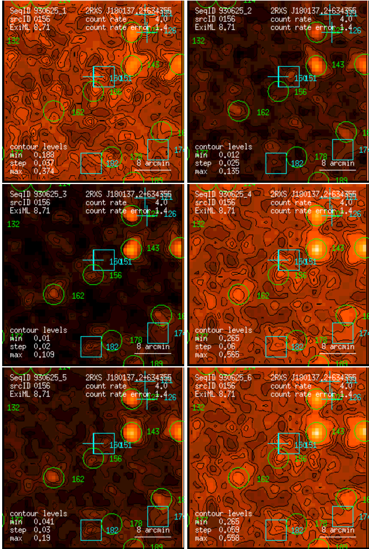
Figure 156: RASS 930625: detection 0156: band rate images, Gaussian filter: (1) PSPC channels 11 – 41, (2) 52 – 90, (3) 91 – 201, (4) 11 – 235, (5) 52 – 201, (6) 11 – 201. Broad band rates in counts/ks. Band rate contour levels in counts/ks/arcmin 2 .
