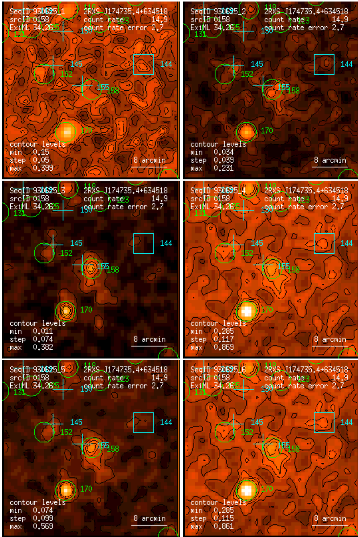
Figure 158: RASS 930625: detection 0158: band rate images, Gaussian filter: (1) PSPC channels 11 – 41, (2) 52 – 90, (3) 91 – 201, (4) 11 – 235, (5) 52 – 201, (6) 11 – 201. Broad band rates in counts/ks. Band rate contour levels in counts/ks/arcmin 2 .
