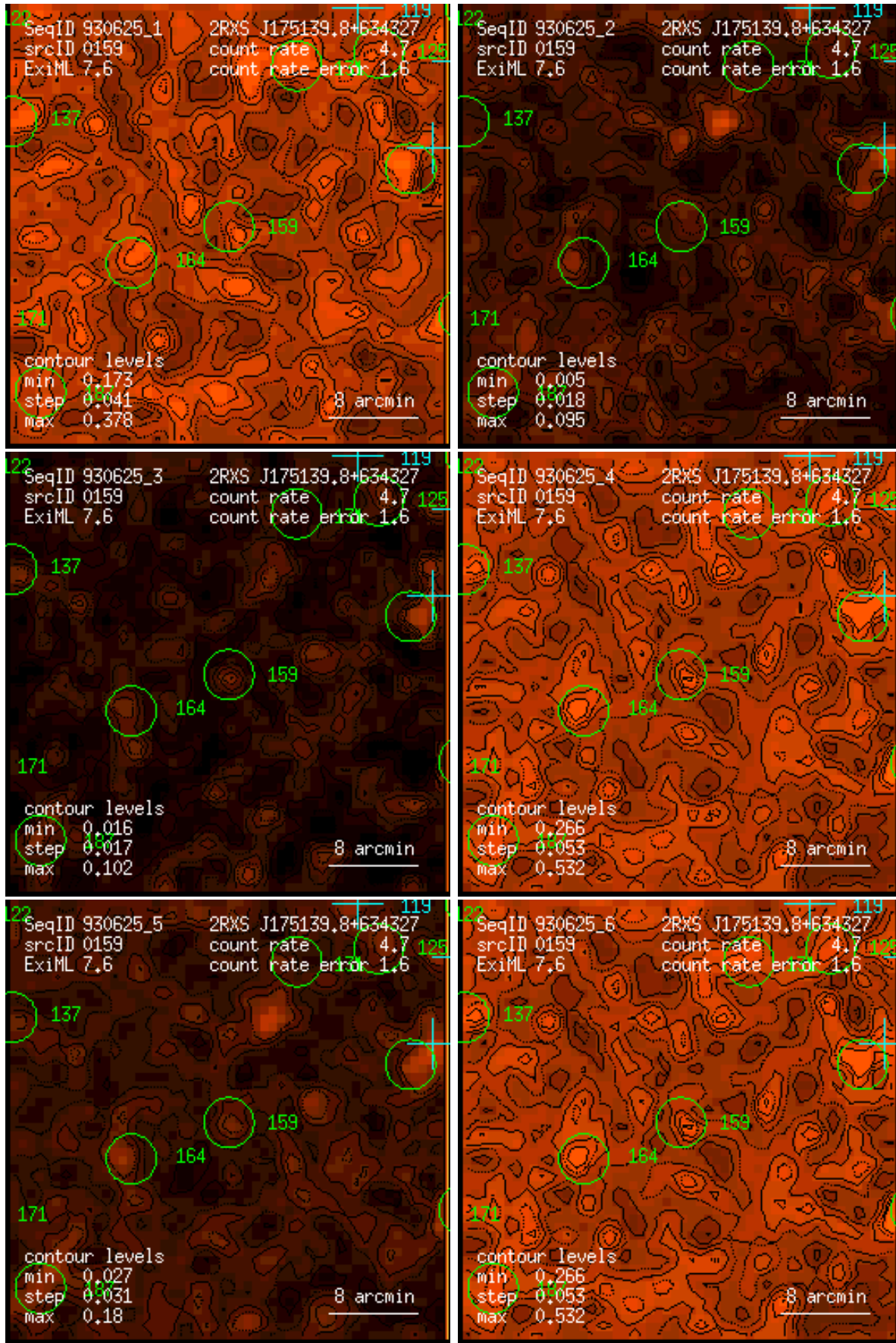
Figure 159: RASS 930625: detection 0159: band rate images, Gaussian filter: (1) PSPC channels 11 – 41, (2) 52 – 90, (3) 91 – 201, (4) 11 – 235, (5) 52 – 201, (6) 11 – 201. Broad band rates in counts/ks. Band rate contour levels in counts/ks/arcmin 2 .
