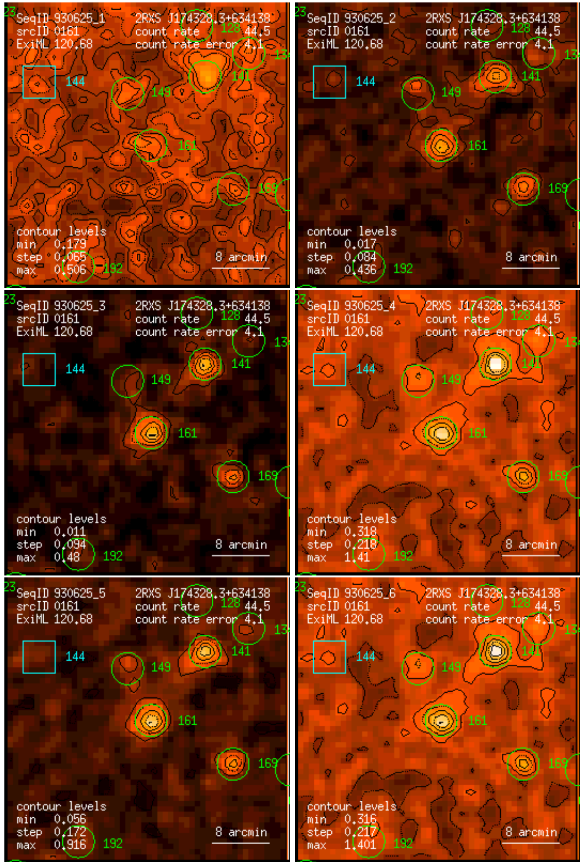
Figure 161: RASS 930625: detection 0161: band rate images, Gaussian filter: (1) PSPC channels 11 – 41, (2) 52 – 90, (3) 91 – 201, (4) 11 – 235, (5) 52 – 201, (6) 11 – 201. Broad band rates in counts/ks. Band rate contour levels in counts/ks/arcmin 2 .
