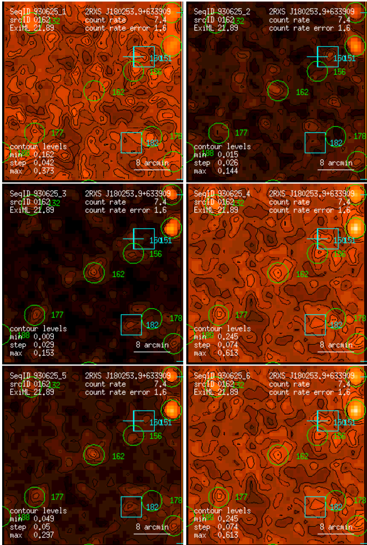
Figure 162: RASS 930625: detection 0162: band rate images, Gaussian filter: (1) PSPC channels 11 – 41, (2) 52 – 90, (3) 91 – 201, (4) 11 – 235, (5) 52 – 201, (6) 11 – 201. Broad band rates in counts/ks. Band rate contour levels in counts/ks/arcmin 2 .
