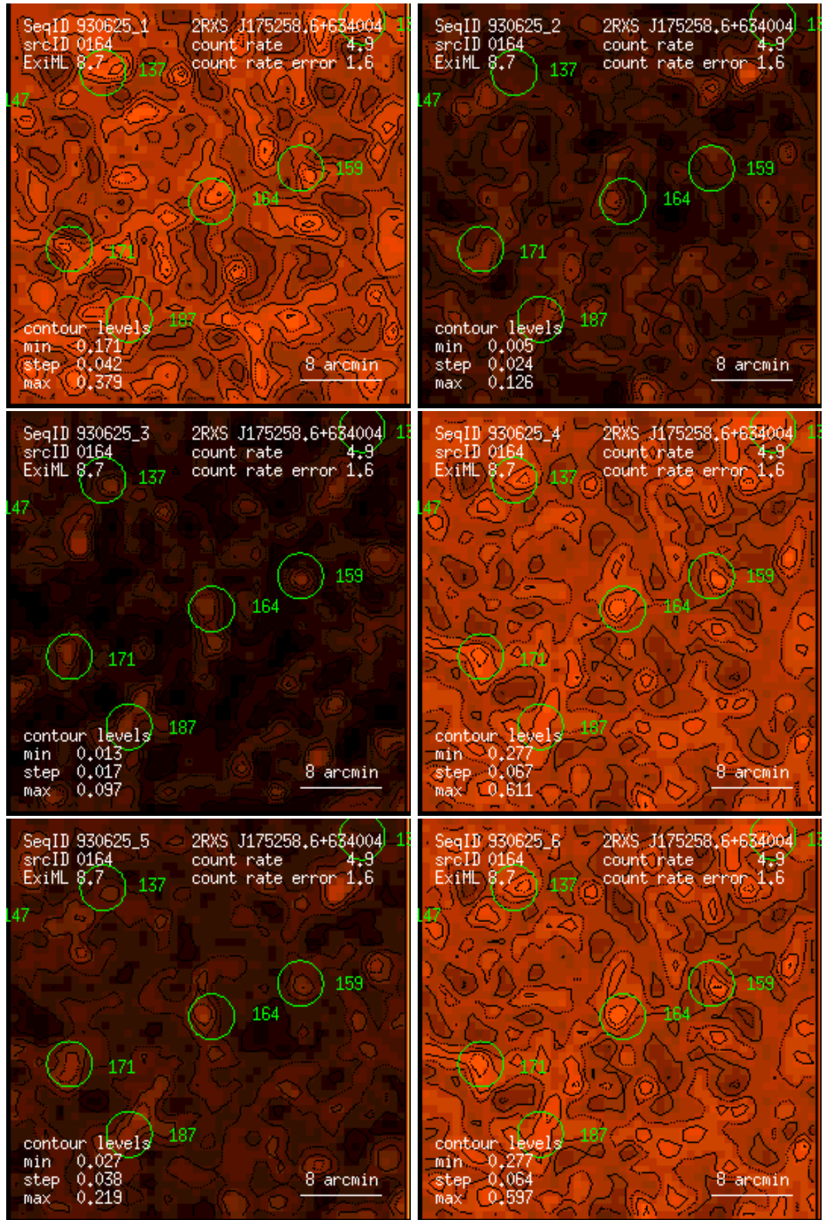
Figure 164: RASS 930625: detection 0164: band rate images, Gaussian filter: (1) PSPC channels 11 – 41, (2) 52 – 90, (3) 91 – 201, (4) 11 – 235, (5) 52 – 201, (6) 11 – 201. Broad band rates in counts/ks. Band rate contour levels in counts/ks/arcmin 2 .
