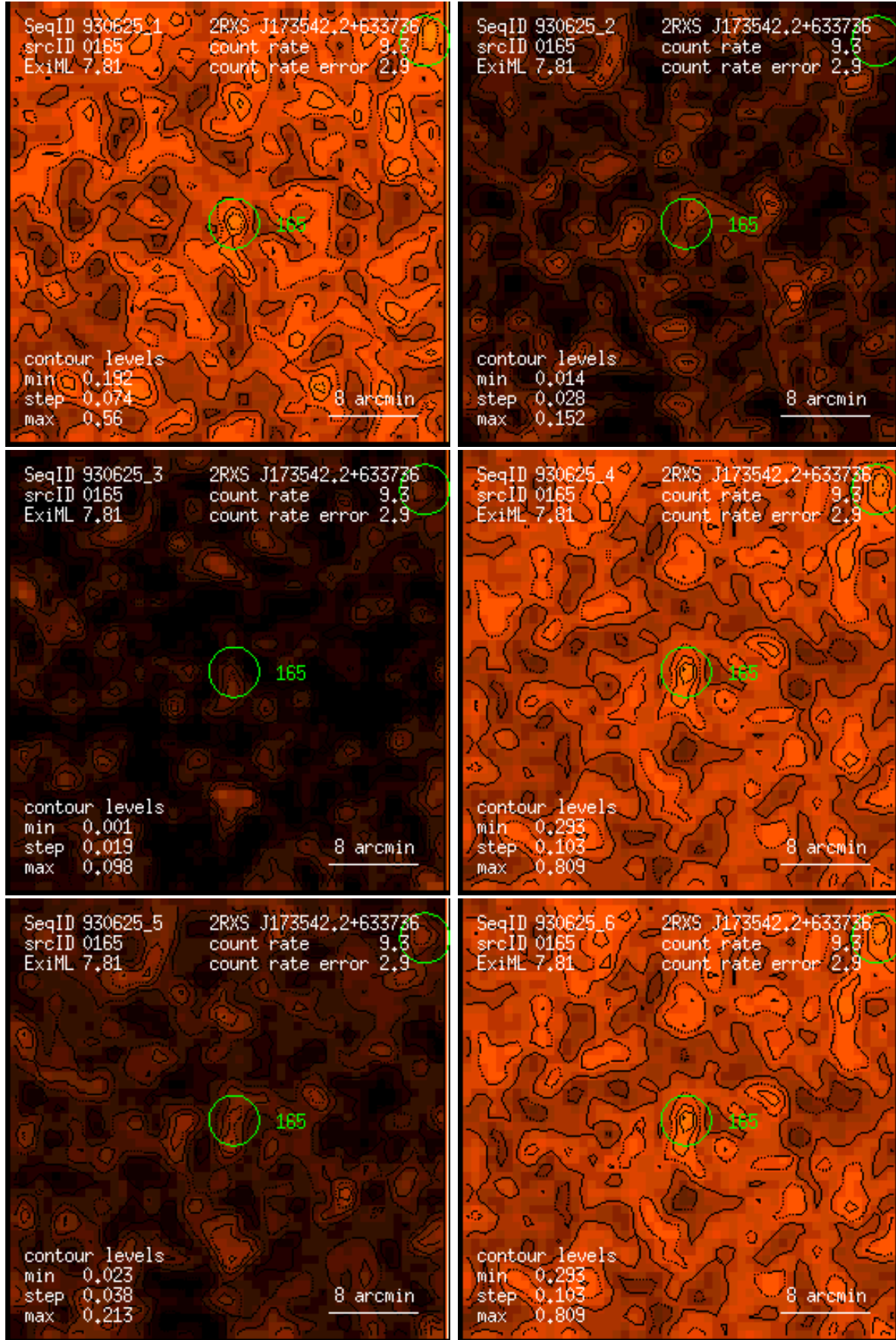
Figure 165: RASS 930625: detection 0165: band rate images, Gaussian filter: (1) PSPC channels 11 – 41, (2) 52 – 90, (3) 91 – 201, (4) 11 – 235, (5) 52 – 201, (6) 11 – 201. Broad band rates in counts/ks. Band rate contour levels in counts/ks/arcmin 2 .
