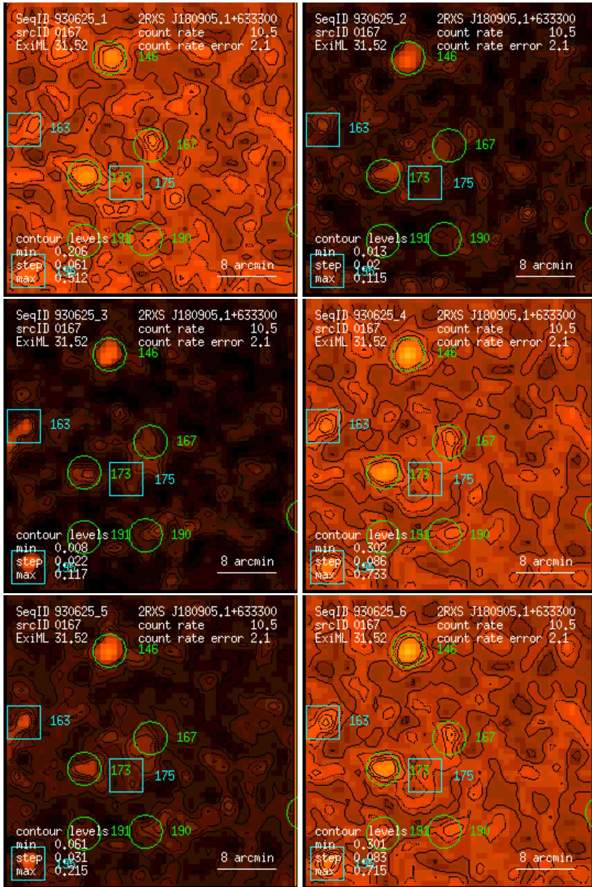
Figure 167: RASS 930625: detection 0167: band rate images, Gaussian filter: (1) PSPC channels 11 – 41, (2) 52 – 90, (3) 91 – 201, (4) 11 – 235, (5) 52 – 201, (6) 11 – 201. Broad band rates in counts/ks. Band rate contour levels in counts/ks/arcmin 2 .
