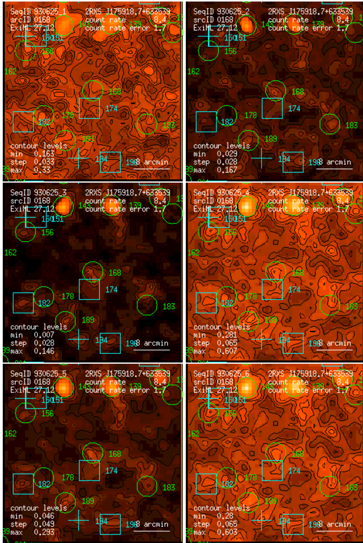
Figure 168: RASS 930625: detection 0168: band rate images, Gaussian filter: (1) PSPC channels 11 – 41, (2) 52 – 90, (3) 91 – 201, (4) 11 – 235, (5) 52 – 201, (6) 11 – 201. Broad band rates in counts/ks. Band rate contour levels in counts/ks/arcmin 2 .
