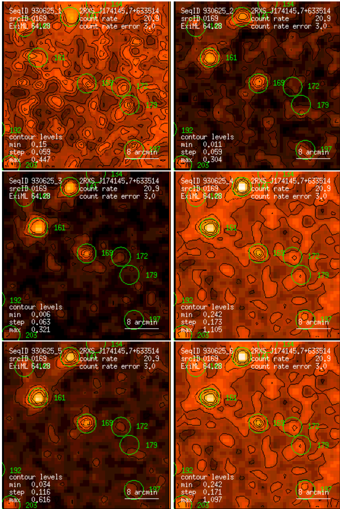
Figure 169: RASS 930625: detection 0169: band rate images, Gaussian filter: (1) PSPC channels 11 – 41, (2) 52 – 90, (3) 91 – 201, (4) 11 – 235, (5) 52 – 201, (6) 11 – 201. Broad band rates in counts/ks. Band rate contour levels in counts/ks/arcmin 2 .
