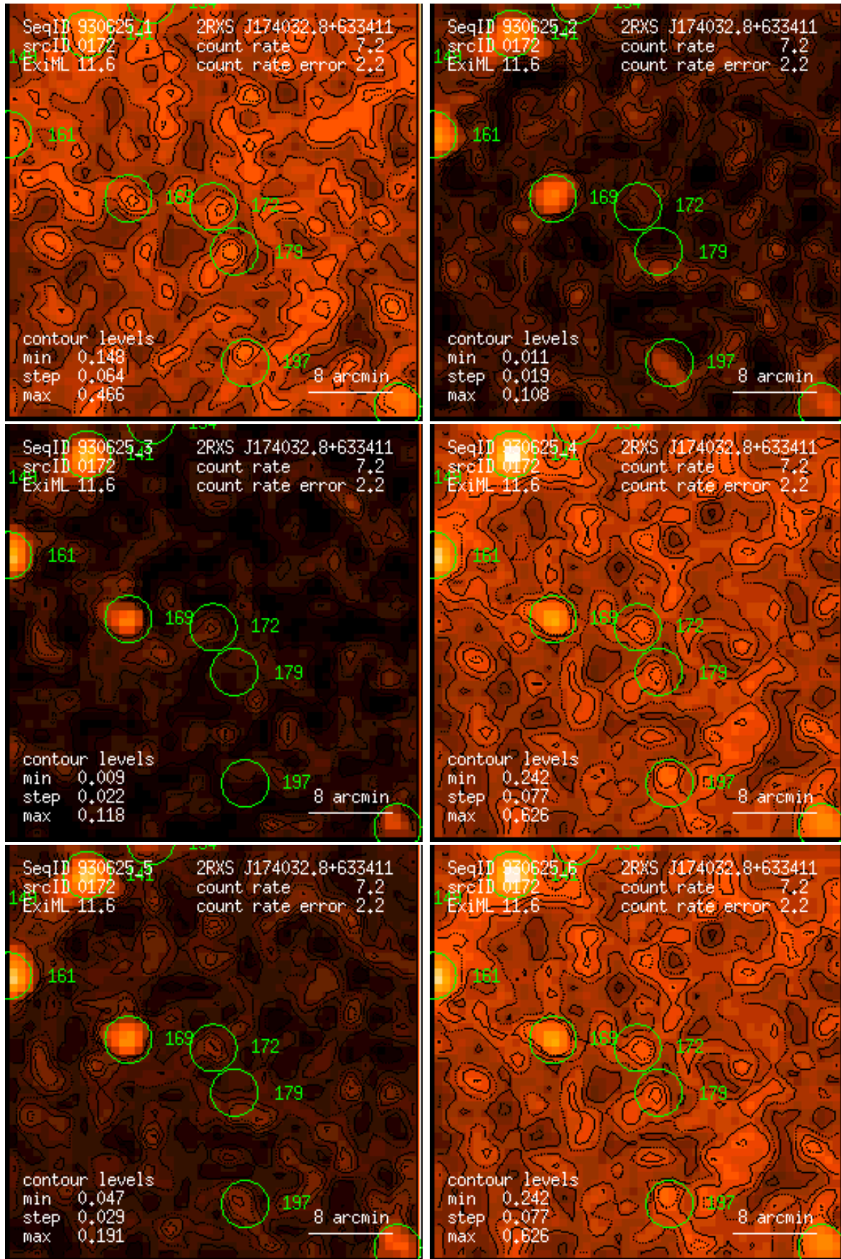
Figure 172: RASS 930625: detection 0172: band rate images, Gaussian filter: (1) PSPC channels 11 – 41, (2) 52 – 90, (3) 91 – 201, (4) 11 – 235, (5) 52 – 201, (6) 11 – 201. Broad band rates in counts/ks. Band rate contour levels in counts/ks/arcmin 2 .
