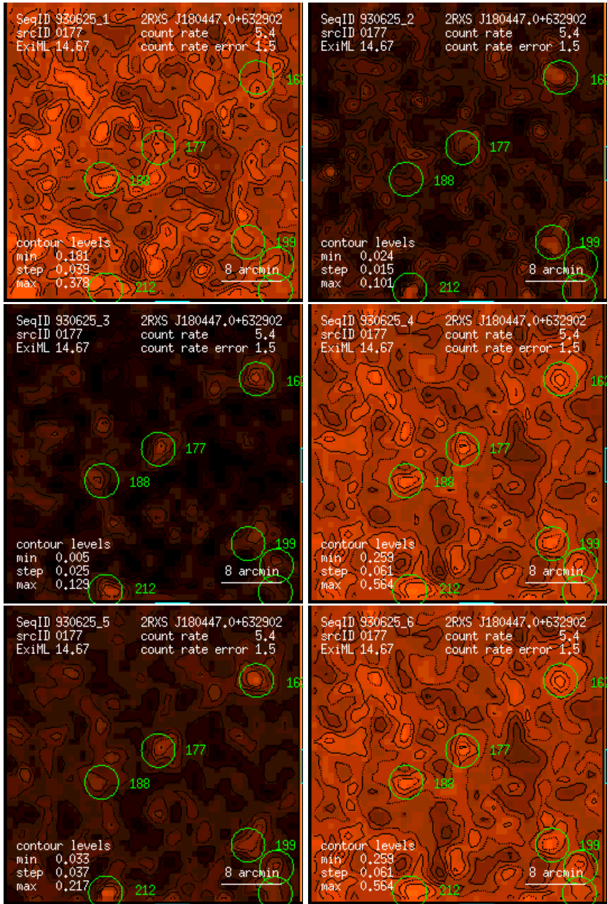
Figure 177: RASS 930625: detection 0177: band rate images, Gaussian filter: (1) PSPC channels 11 – 41, (2) 52 – 90, (3) 91 – 201, (4) 11 – 235, (5) 52 – 201, (6) 11 – 201. Broad band rates in counts/ks. Band rate contour levels in counts/ks/arcmin 2 .
