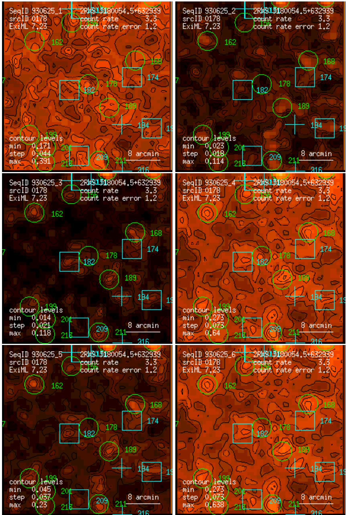
Figure 178: RASS 930625: detection 0178: band rate images, Gaussian filter: (1) PSPC channels 11 – 41, (2) 52 – 90, (3) 91 – 201, (4) 11 – 235, (5) 52 – 201, (6) 11 – 201. Broad band rates in counts/ks. Band rate contour levels in counts/ks/arcmin 2 .
