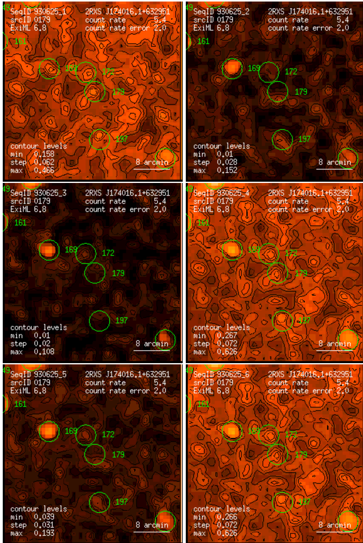
Figure 179: RASS 930625: detection 0179: band rate images, Gaussian filter: (1) PSPC channels 11 – 41, (2) 52 – 90, (3) 91 – 201, (4) 11 – 235, (5) 52 – 201, (6) 11 – 201. Broad band rates in counts/ks. Band rate contour levels in counts/ks/arcmin 2 .
