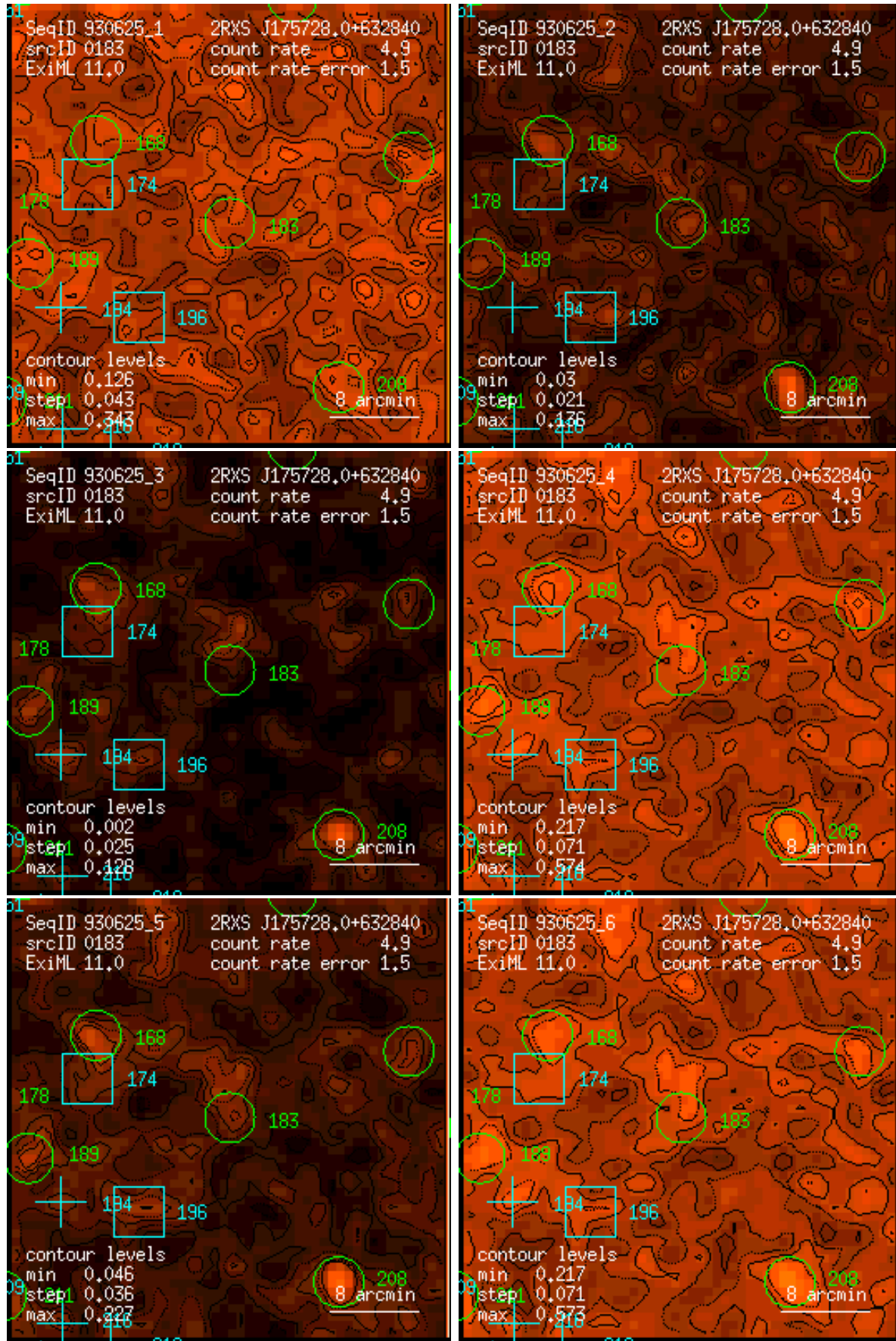
Figure 183: RASS 930625: detection 0183: band rate images, Gaussian filter: (1) PSPP channels 11 – 41, (2) 52 – 90, (3) 91 – 201, (4) 11 – 235, (5) 52 – 201, (6) 11 – 201. Broad band rates in counts/ks. Band rate contour levels in counts/ks/arcmin 2 .
