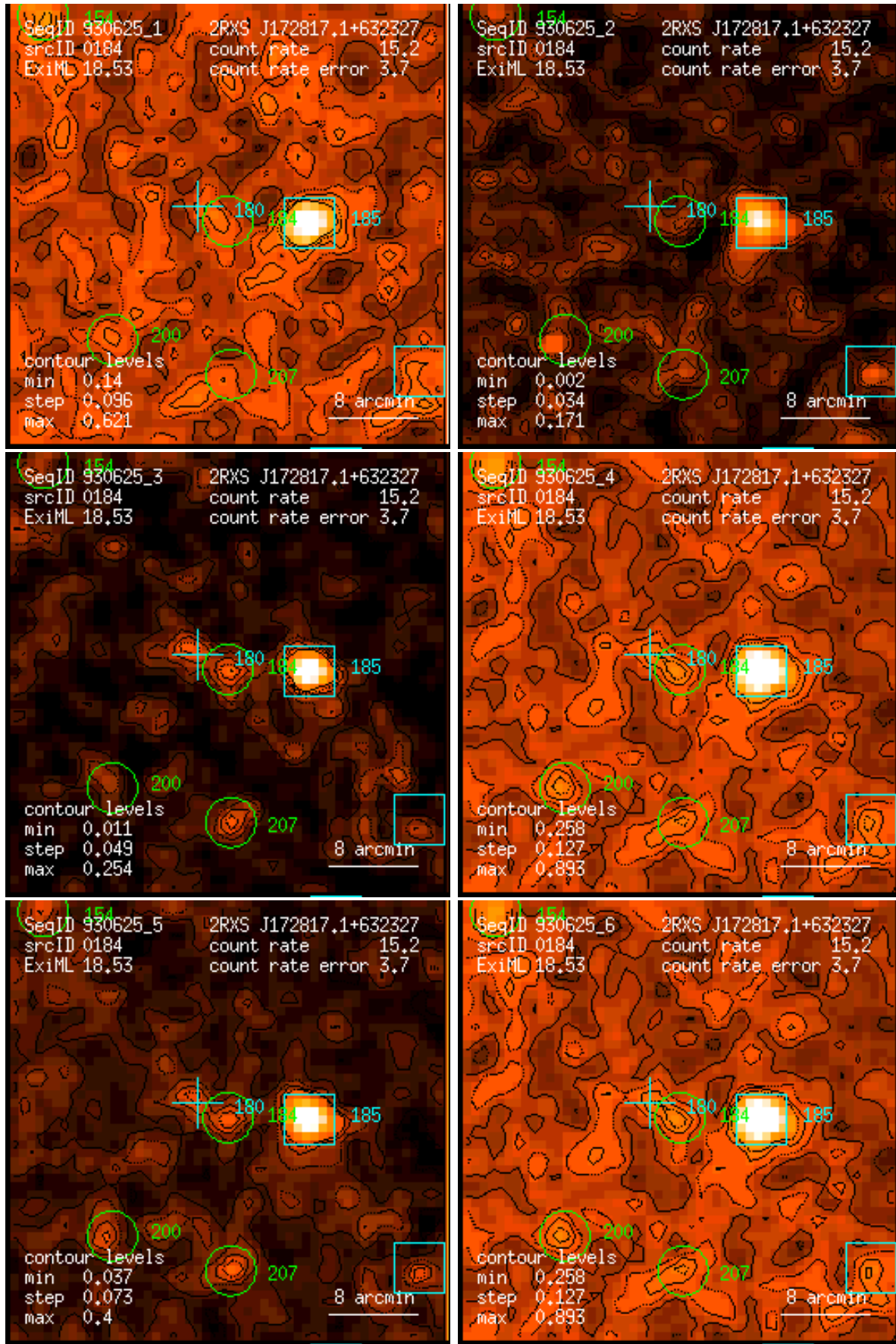
Figure 184: RASS 930625: detection 0184: band rate images, Gaussian filter: (1) PSPC channels 11 – 41, (2) 52 – 90, (3) 91 – 201, (4) 11 – 235, (5) 52 – 201, (6) 11 – 201. Broad band rates in counts/ks. Band rate contour levels in counts/ks/arcmin 2 .
