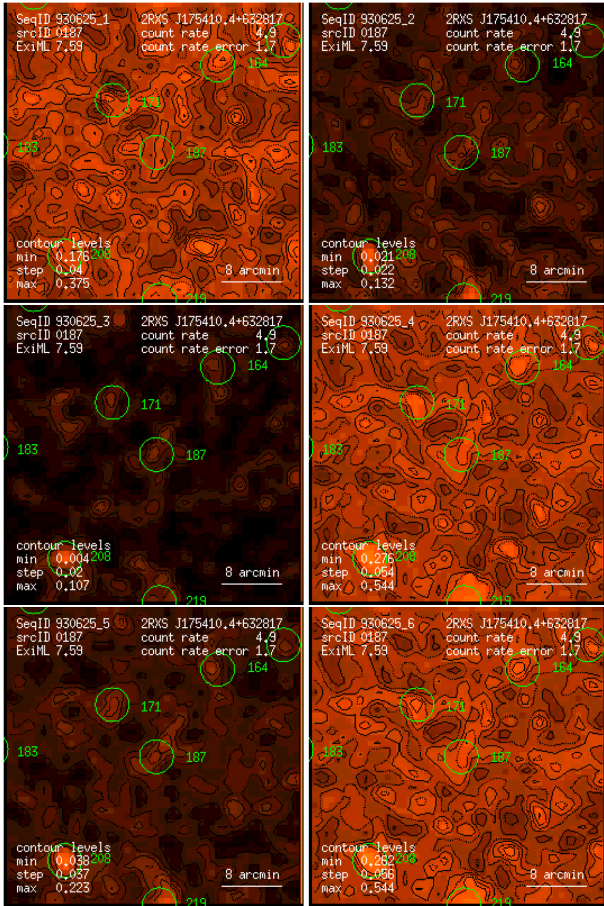
Figure 187: RASS 930625: detection 0187: band rate images, Gaussian filter: (1) PSPC channels 11 – 41, (2) 52 – 90, (3) 91 – 201, (4) 11 – 235, (5) 52 – 201, (6) 11 – 201. Broad band rates in counts/ks. Band rate contour levels in counts/ks/arcmin 2 .
