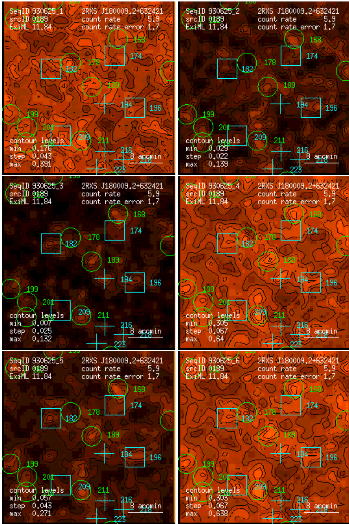
Figure 189: RASS 930625: detection 0189: band rate images, Gaussian filter: (1) PSPC channels 11 – 41, (2) 52 – 90, (3) 91 – 201, (4) 11 – 235, (5) 52 – 201, (6) 11 – 201. Broad band rates in counts/ks. Band rate contour levels in counts/ks/arcmin 2 .
