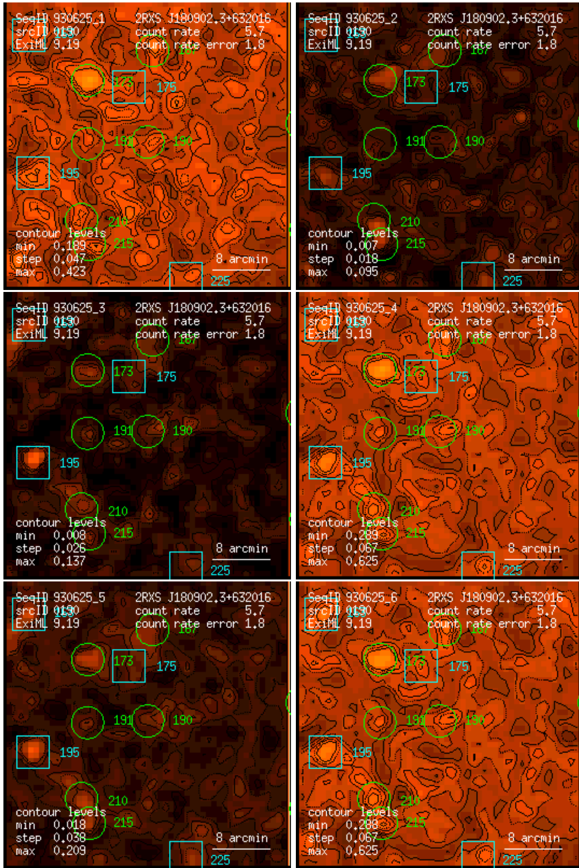
Figure 190: RASS 930625: detection 0190: band rate images, Gaussian filter: (1) PSPC channels 11 – 41, (2) 52 – 90, (3) 91 – 201, (4) 11 – 235, (5) 52 – 201, (6) 11 – 201. Broad band rates in counts/ks. Band rate contour levels in counts/ks/arcmin 2 .
