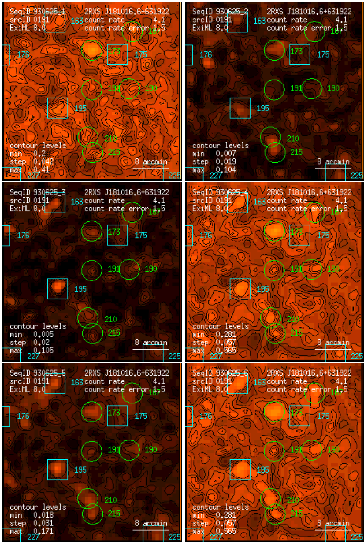
Figure 191: RASS 930625: detection 0191: band rate images, Gaussian filter: (1) PSPC channels 11 – 41, (2) 52 – 90, (3) 91 – 201, (4) 11 – 235, (5) 52 – 201, (6) 11 – 201. Broad band rates in counts/ks. Band rate contour levels in counts/ks/arcmin 2 .
