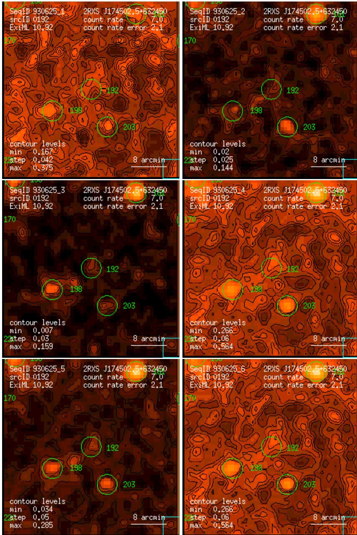
Figure 192: RASS 930625: detection 0192: band rate images, Gaussian filter: (1) PSPC channels 11 – 41, (2) 52 – 90, (3) 91 – 201, (4) 11 – 235, (5) 52 – 201, (6) 11 – 201. Broad band rates in counts/ks. Band rate contour levels in counts/ks/arcmin 2 .
