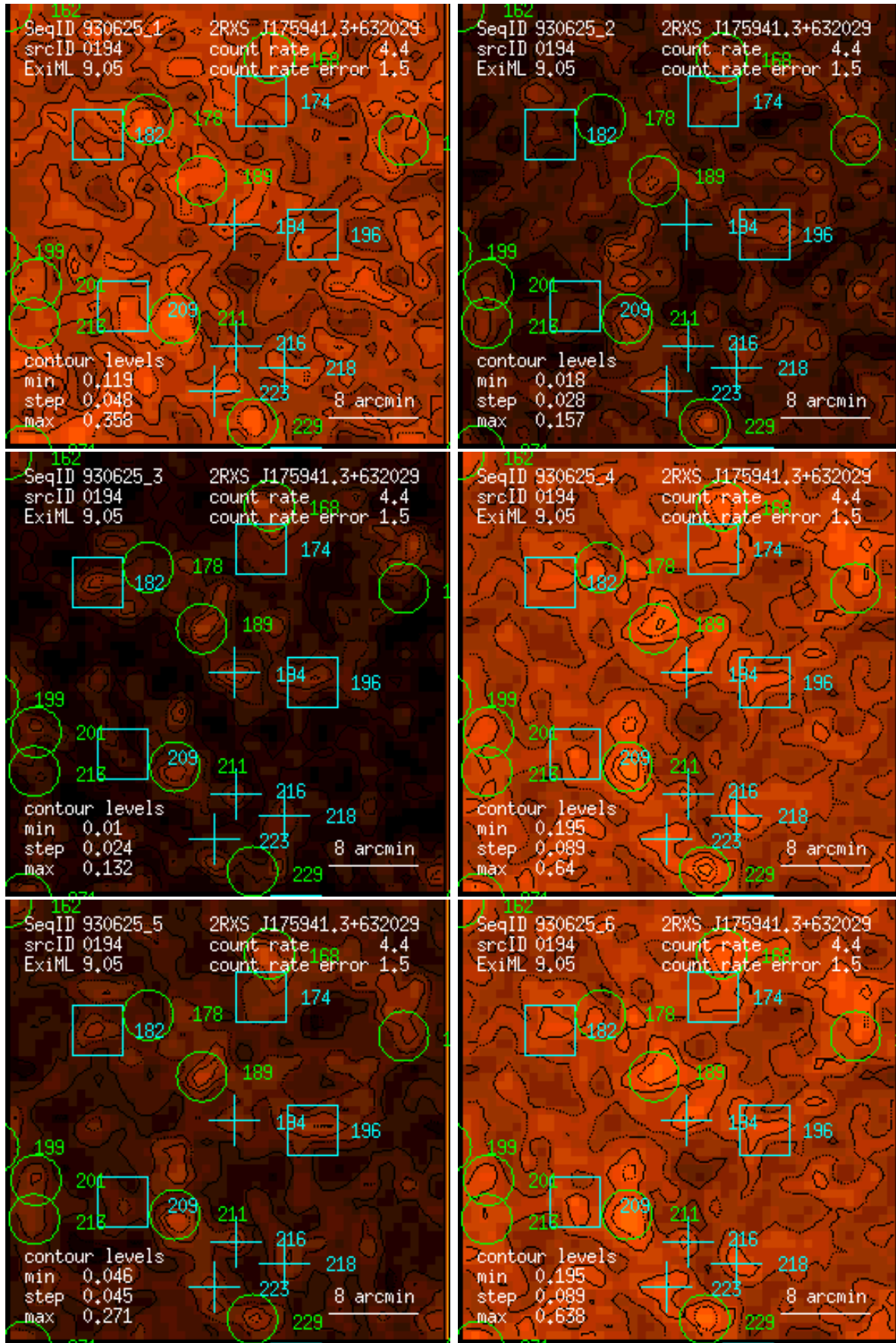
Figure 194: RASS 930625: detection 0194: band rate images, Gaussian filter: (1) PSPC channels 11 – 41, (2) 52 – 90, (3) 91 – 201, (4) 11 – 235, (5) 52 – 201, (6) 11 – 201. Broad band rates in counts/ks. Band rate contour levels in counts/ks/arcmin 2 .
