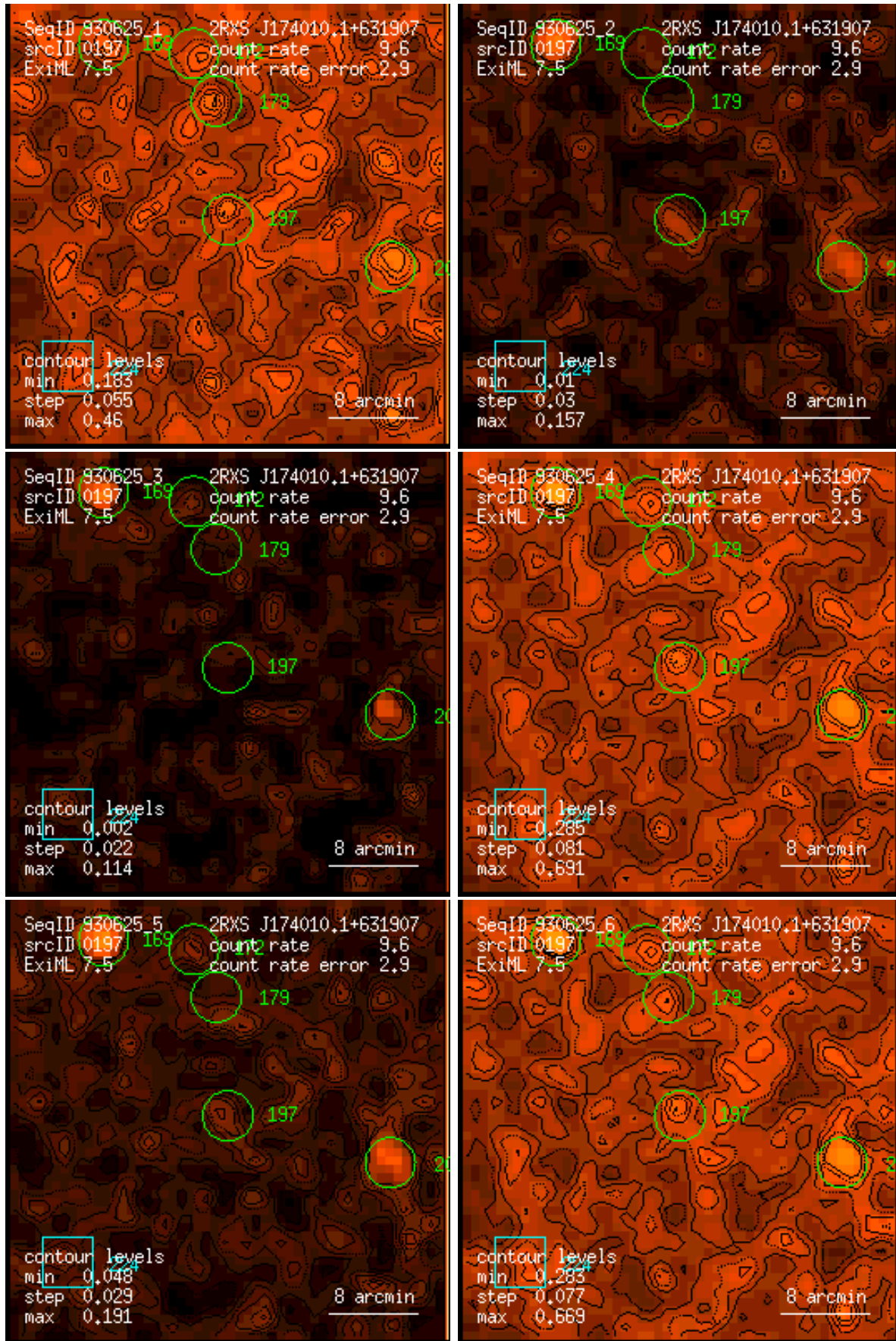
Figure 197: RASS 930625: detection 0197: band rate images, Gaussian filter: (1) PSPC channels 11 – 41, (2) 52 – 90, (3) 91 – 201, (4) 11 – 235, (5) 52 – 201, (6) 11 – 201. Broad band rates in counts/ks. Band rate contour levels in counts/ks/arcmin 2 .
