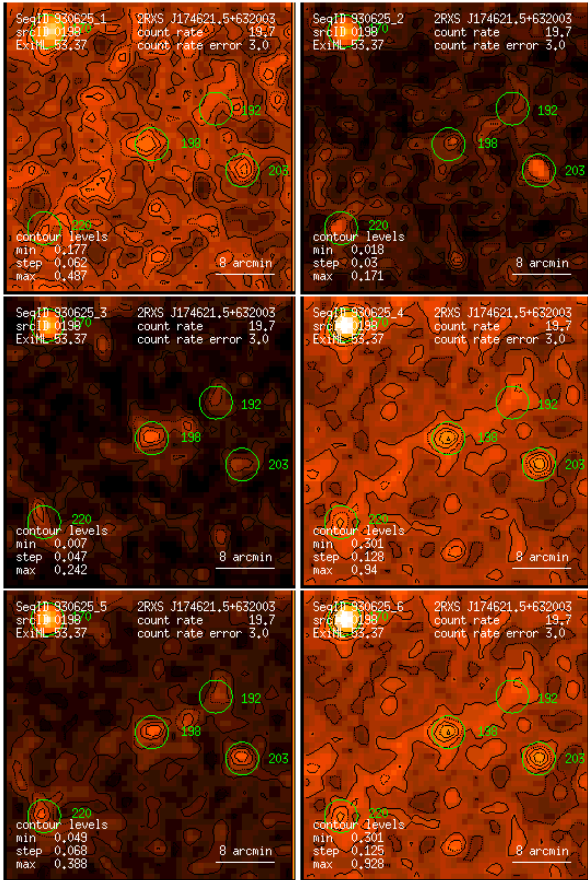
Figure 198: RASS 930625: detection 0198: band rate images, Gaussian filter: (1) PSPC channels 11 – 41, (2) 52 – 90, (3) 91 – 201, (4) 11 – 235, (5) 52 – 201, (6) 11 – 201. Broad band rates in counts/ks. Band rate contour levels in counts/ks/arcmin 2 .
