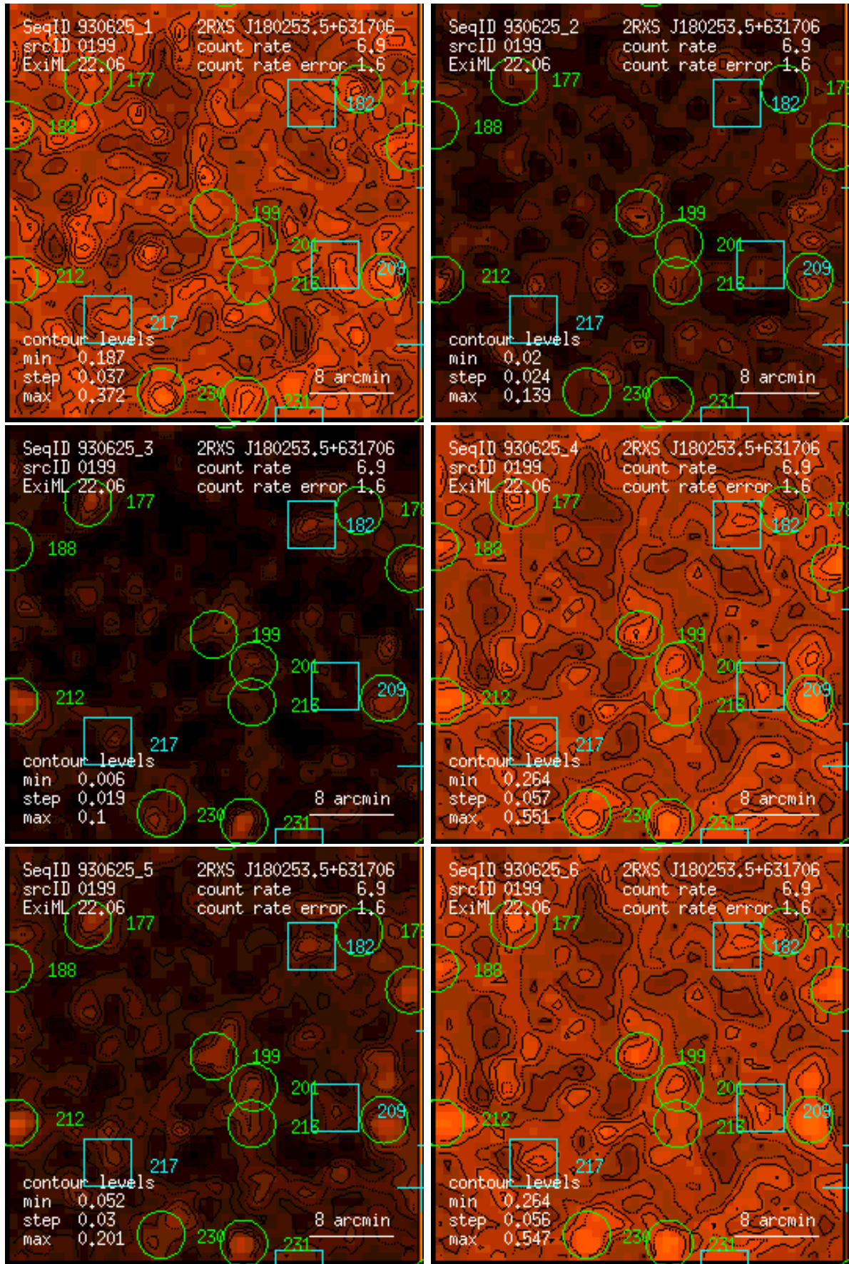
Figure 199: RASS 930625: detection 0199: band rate images, Gaussian filter: (1) PSPC channels 11 – 41, (2) 52 – 90, (3) 91 – 201, (4) 11 – 235, (5) 52 – 201, (6) 11 – 201. Broad band rates in counts/ks. Band rate contour levels in counts/ks/arcmin 2 .
