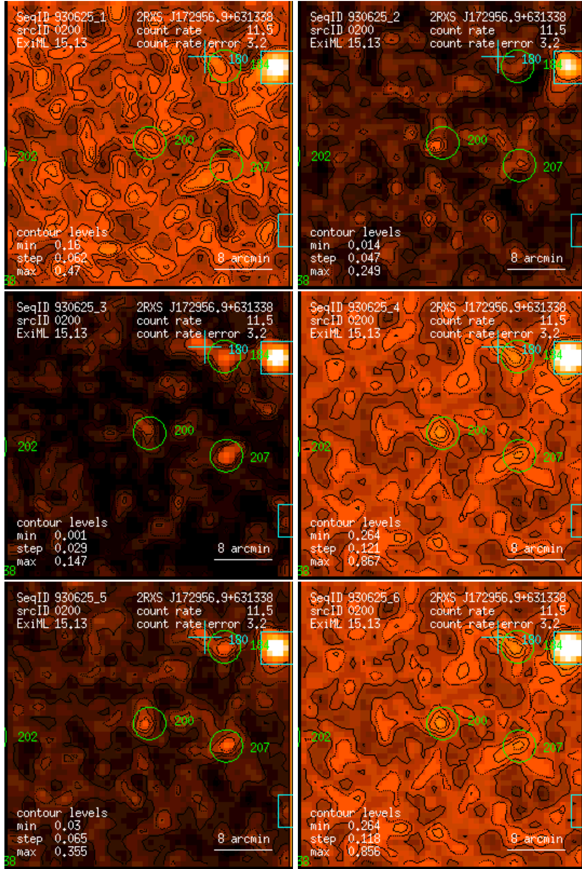
Figure 200: RASS 930625: detection 0200: band rate images, Gaussian filter: (1) PSPC channels 11 – 41, (2) 52 – 90, (3) 91 – 201, (4) 11 – 235, (5) 52 – 201, (6) 11 – 201. Broad band rates in counts/ks. Band rate contour levels in counts/ks/arcmin 2 .
