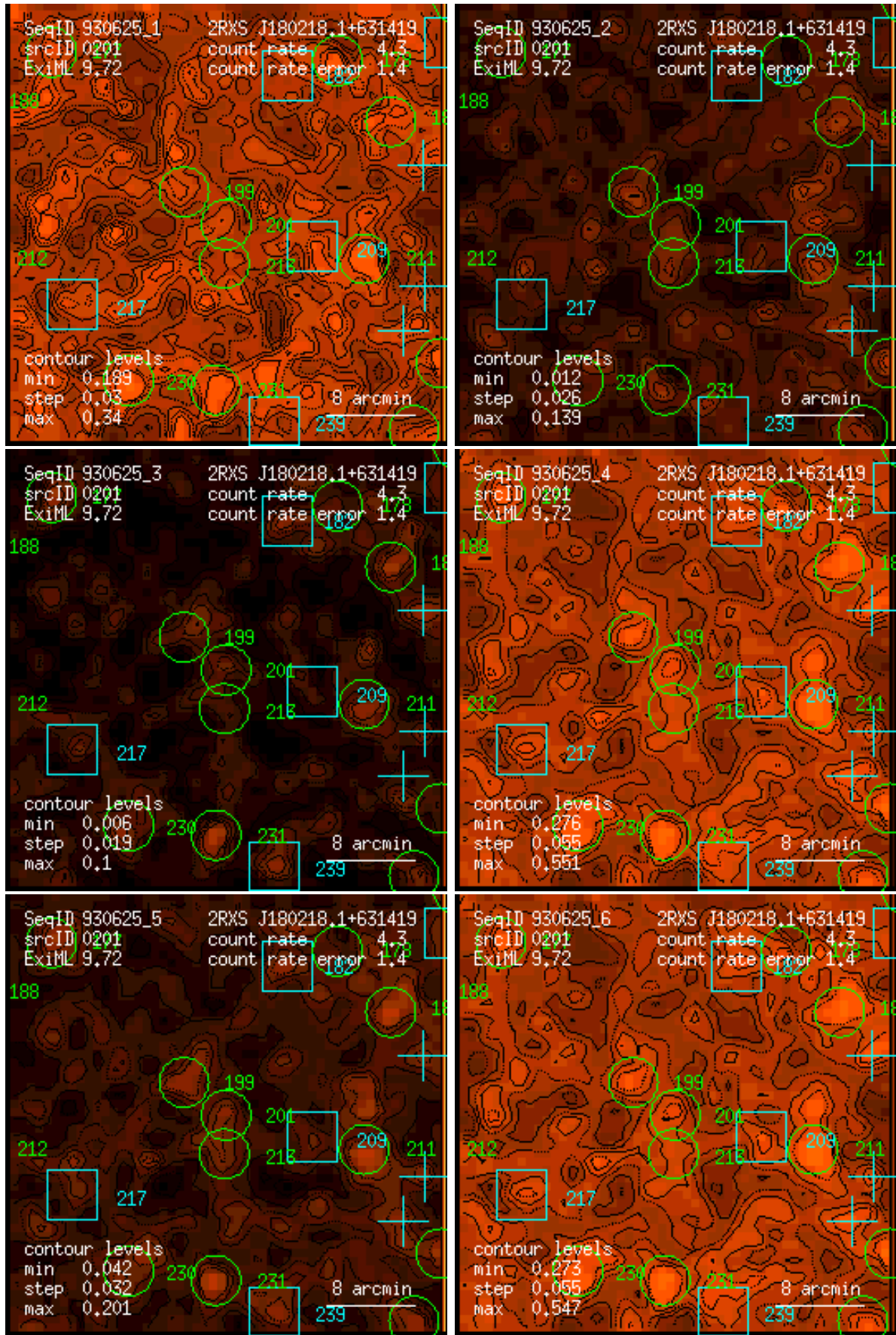
Figure 201: RASS 930625: detection 0201: band rate images, Gaussian filter: (1) PSPC channels 11 – 41, (2) 52 – 90, (3) 91 – 201, (4) 11 – 235, (5) 52 – 201, (6) 11 – 201. Broad band rates in counts/ks. Band rate contour levels in counts/ks/arcmin 2 .
